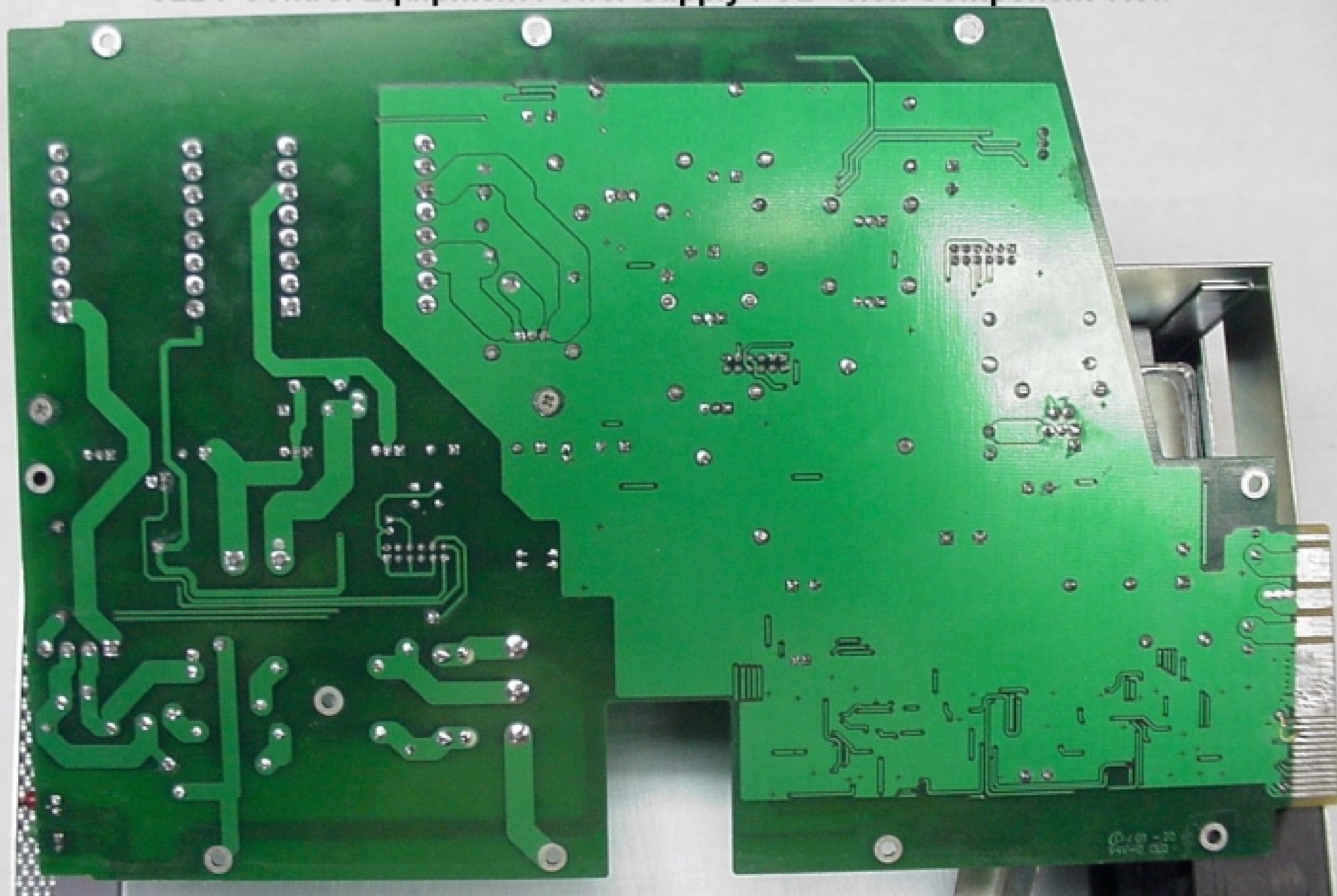
G2BT Control Equipment Power Supply PCB - Non Component View
