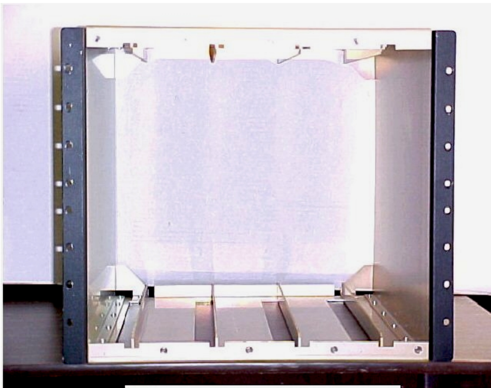
G2BT Amplifier Chassis (Secures 4 AML Amplifiers)
