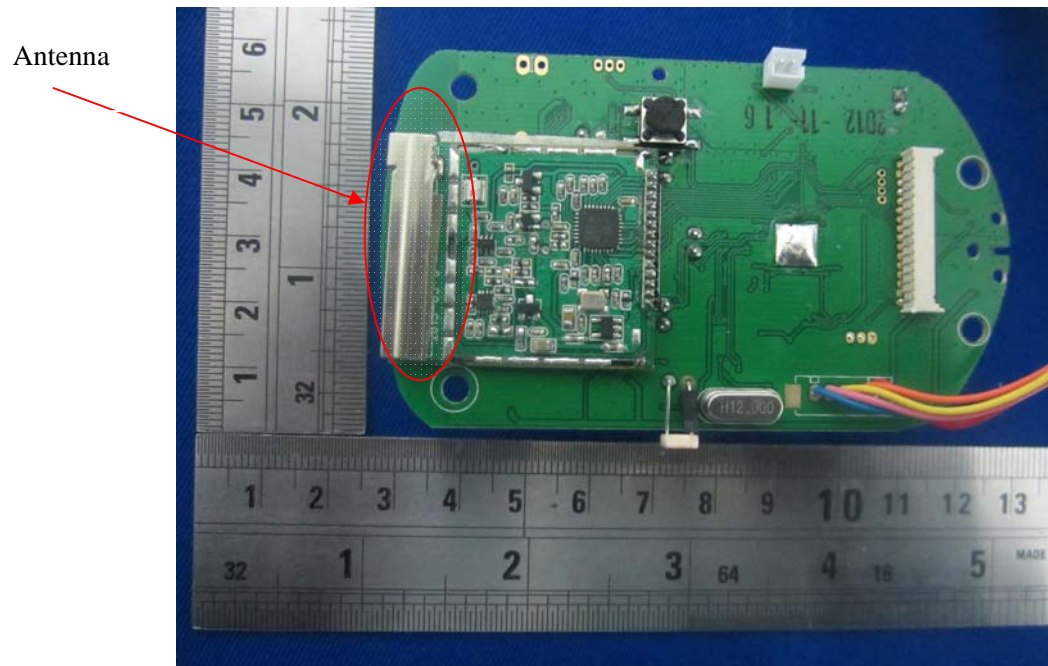
EUT – Main Board Bottom Without Shielding View
