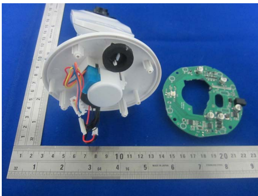
EUT – Control Cover Off View
