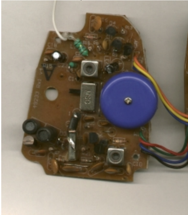
Internal PCB Component side
