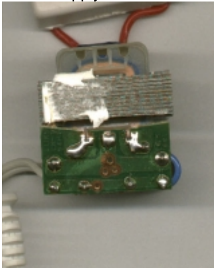
Power Supply Foil side
