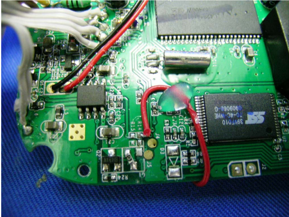
Baby Unit Main PCB rear side (View 3)
