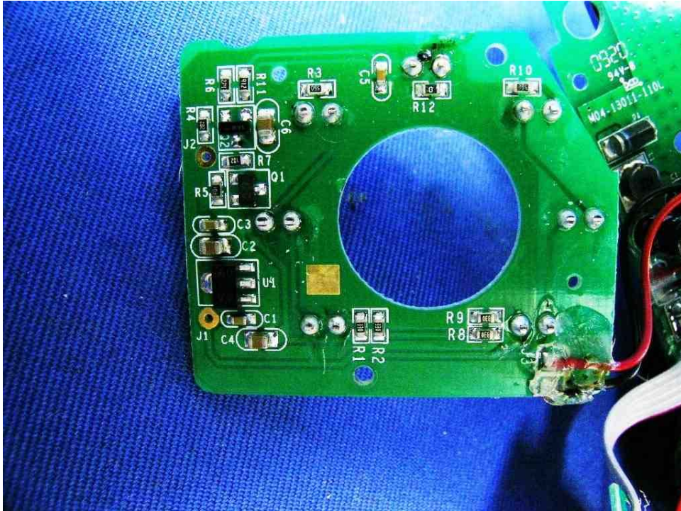
Baby Unit LED PCB rear side
