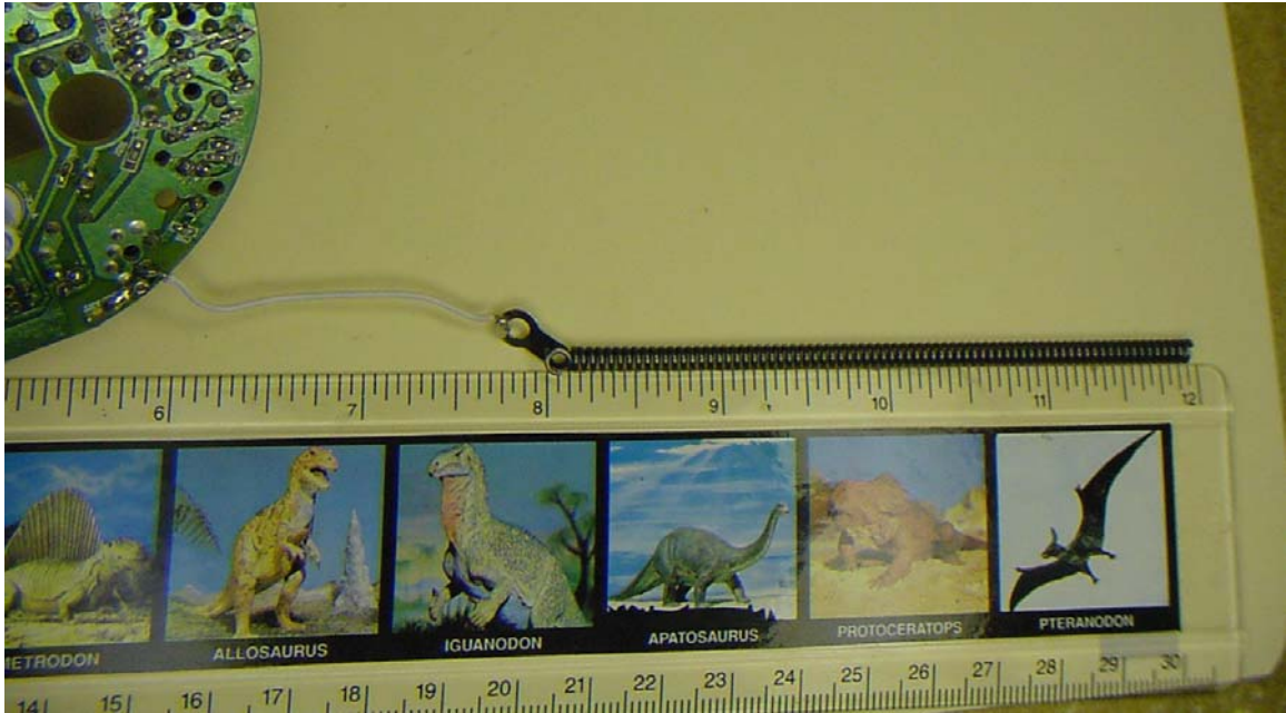
Antenna system, soldered wire at the PCB, the connector and antenna are screwed together onto the housing of the EUT.
