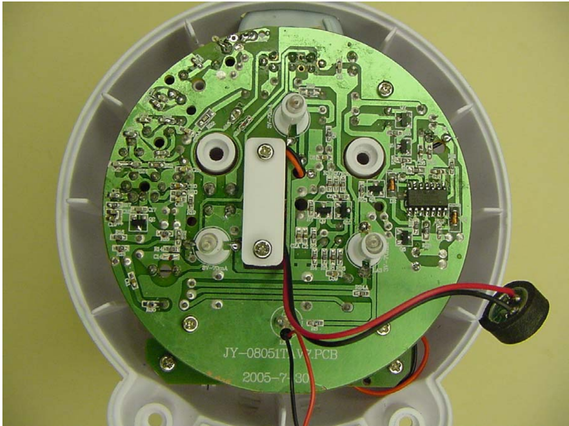
PCB Rear
