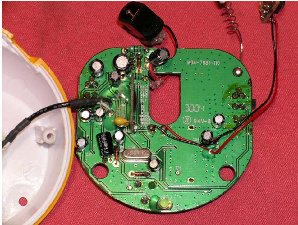
Base Main PCB rear side (View 1)
