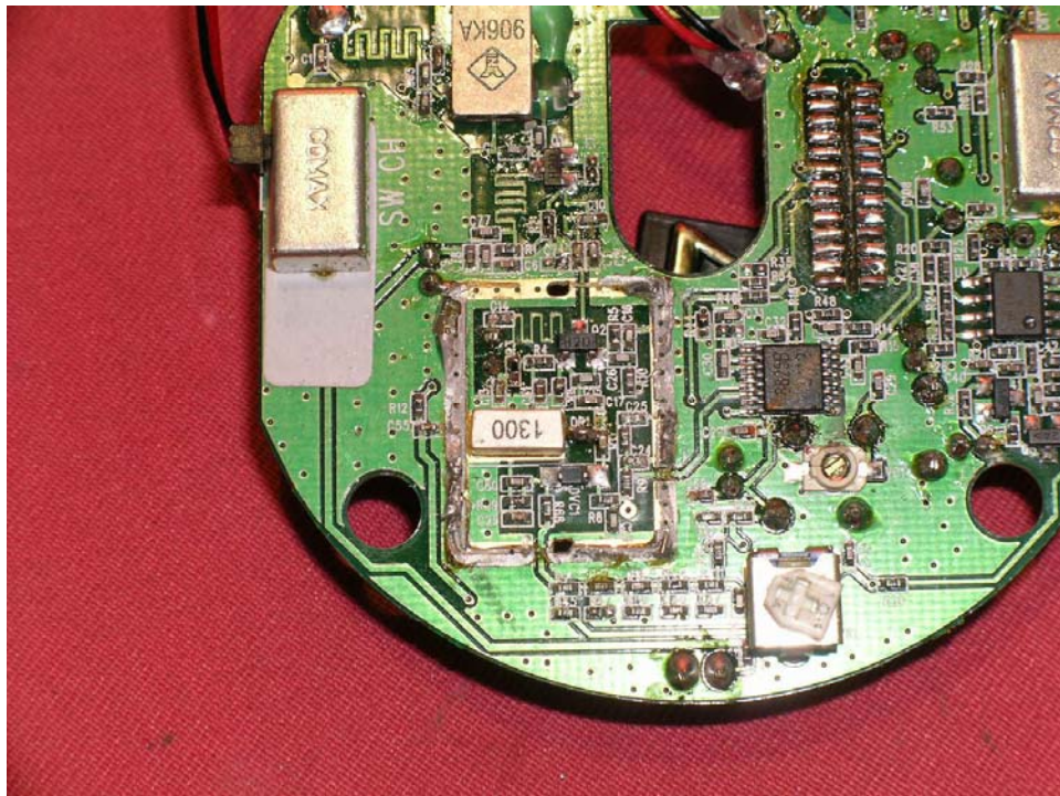
Base Main PCB front side (View 2)
