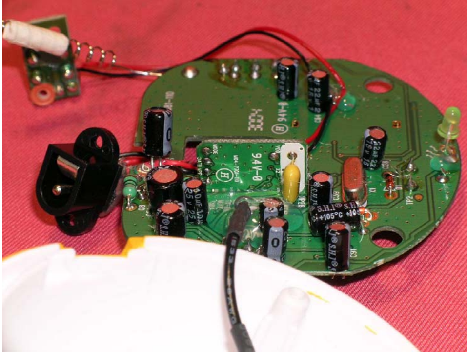
Base Main PCB rear side (View 3)
