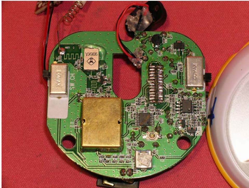
Base Main PCB front side (View 1)
