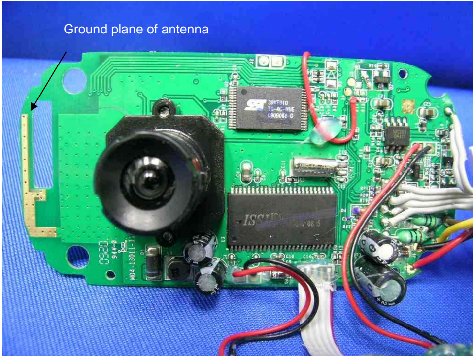
Baby Unit Main PCB rear side (View 1)
