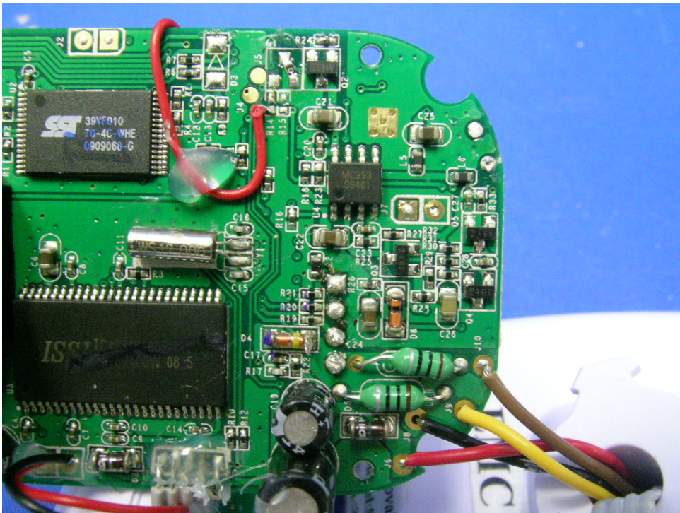
Baby Unit Main PCB rear side (View 2)
