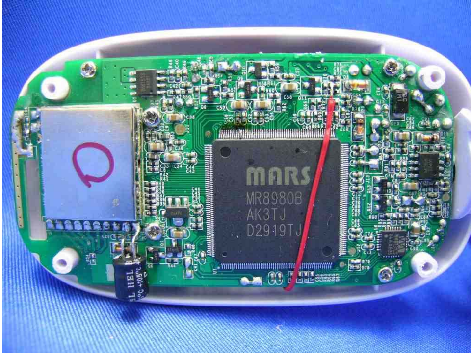
Baby Unit Main PCB front side (View 1)
