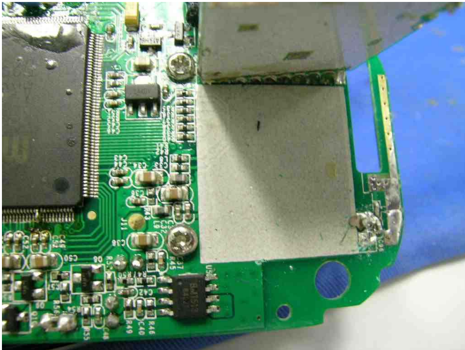
Baby Unit Main PCB front side (View 2)
