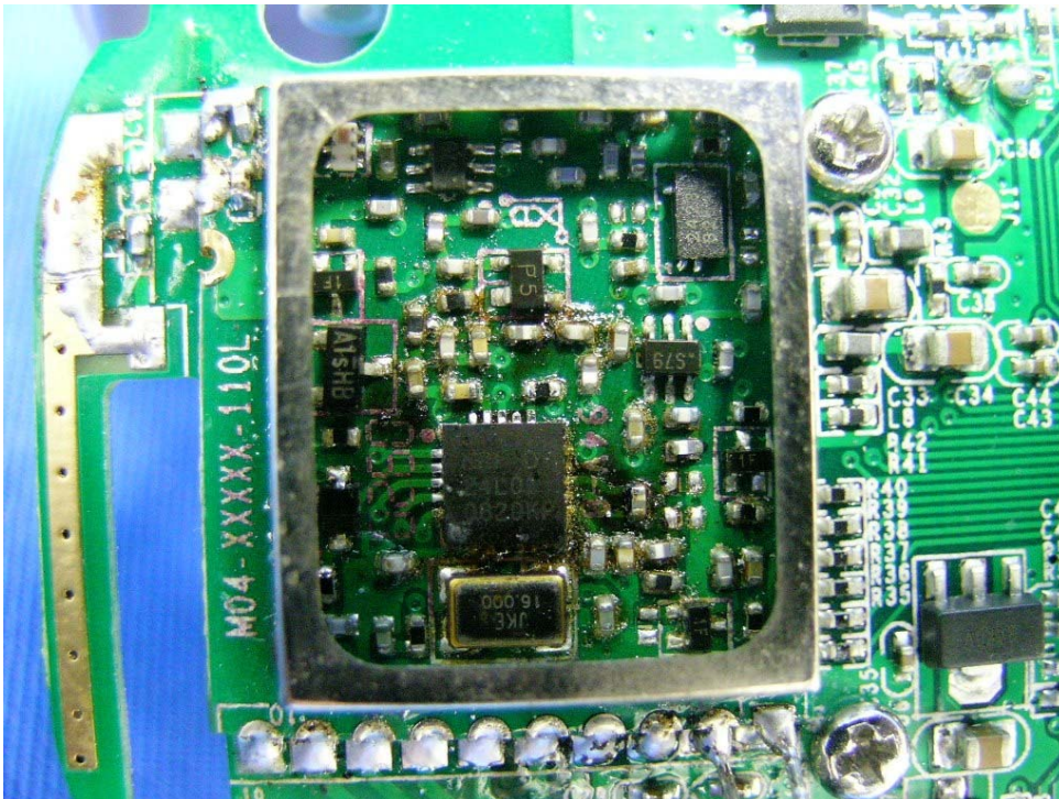
Baby Unit RF Module PCB front side
