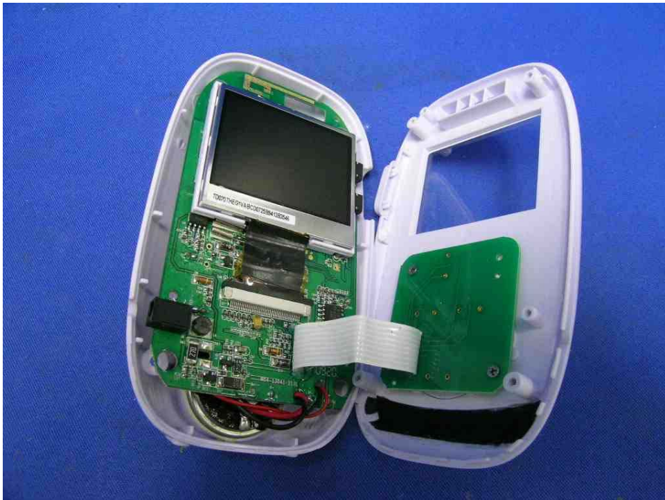
Parent Unit assembly (View 2)
