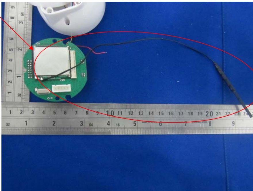
EUT – Camera Board Bottom With Shielding View
