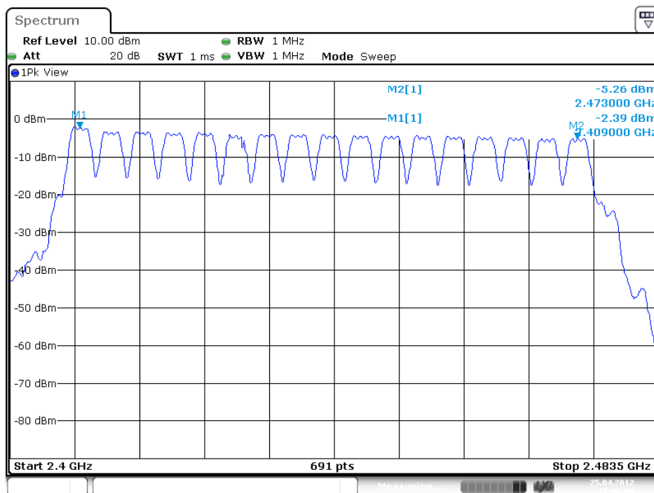
Number of Hopping Channel Plot on Channel 1~17 / 2409 MHz ~ 2473 MHz
