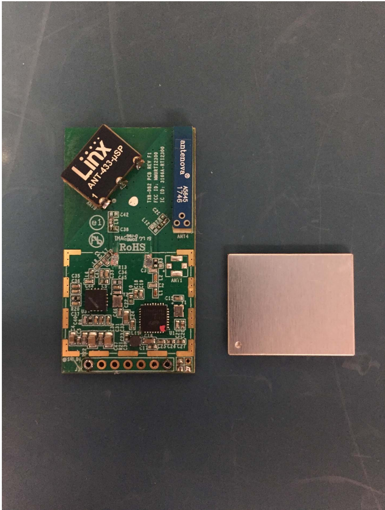
TXB-DB2 Module Top without Shield
