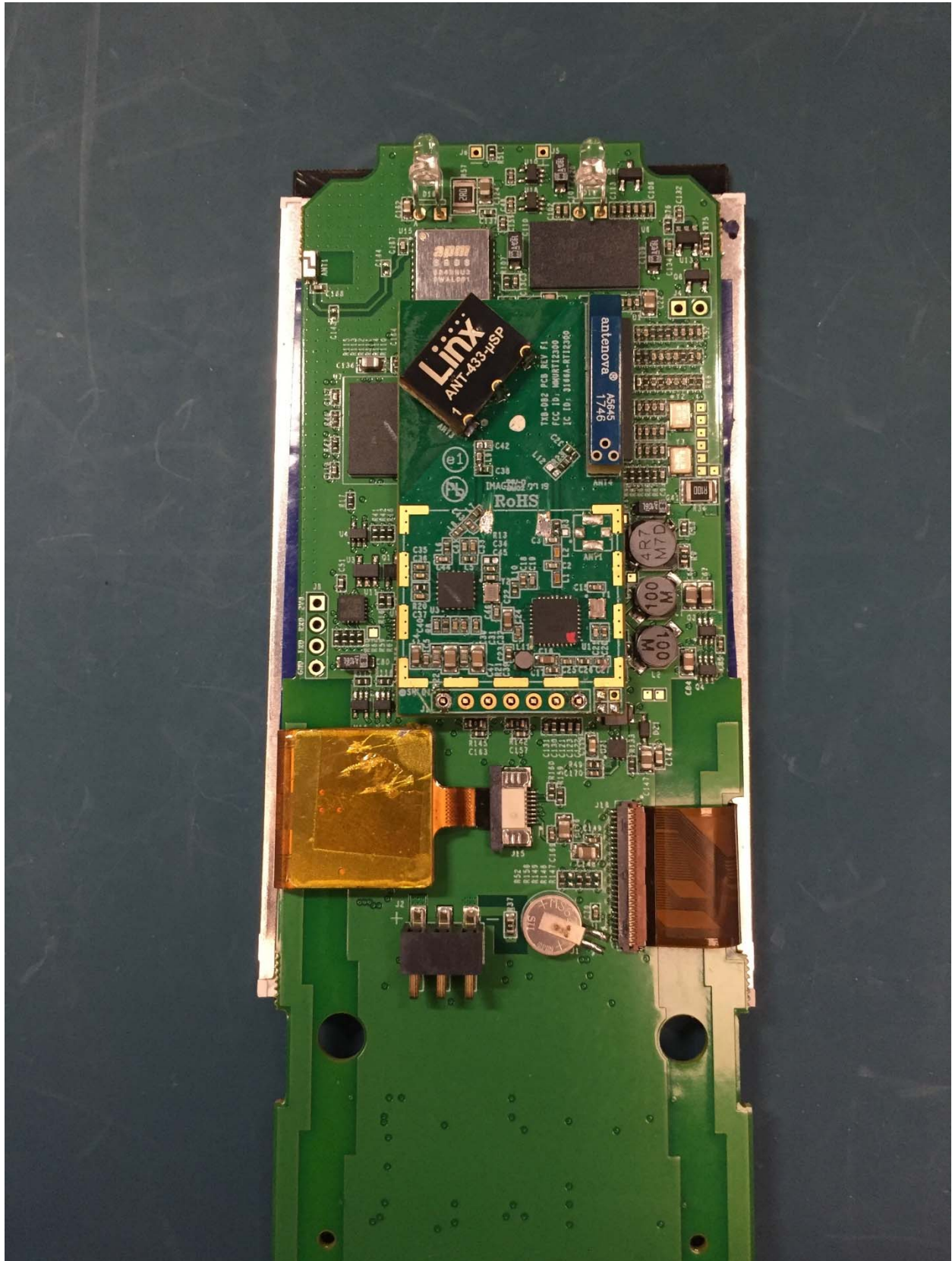
TXB-DB2 Host Fixture 2
