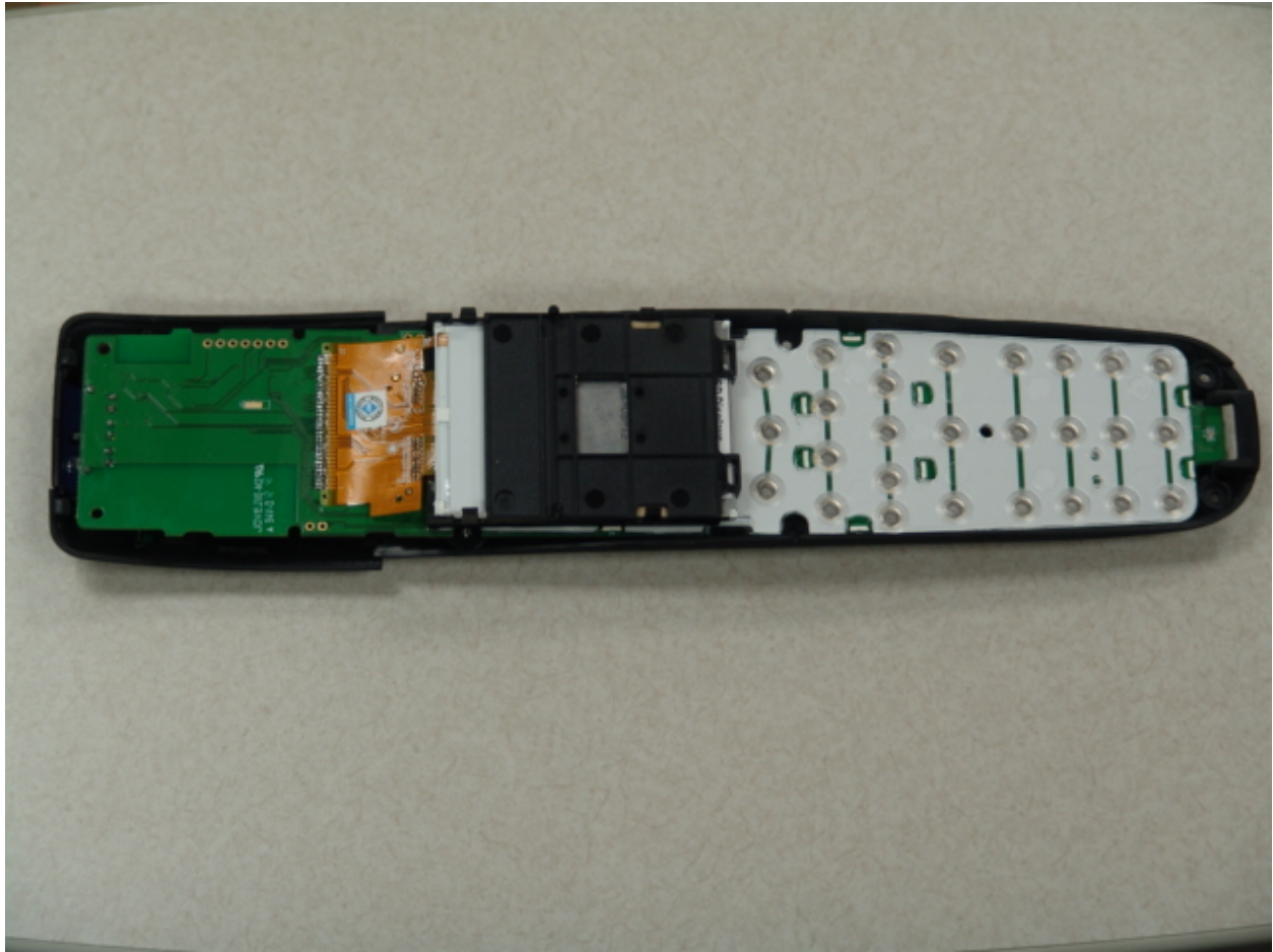
Top of PCB under LCD
