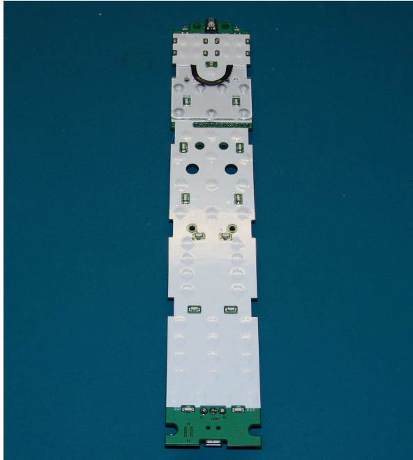
T1-B PCB – Front
