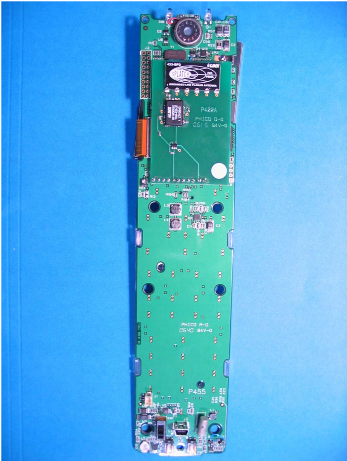
Figure 3: Main and Daughter Board Bottom
