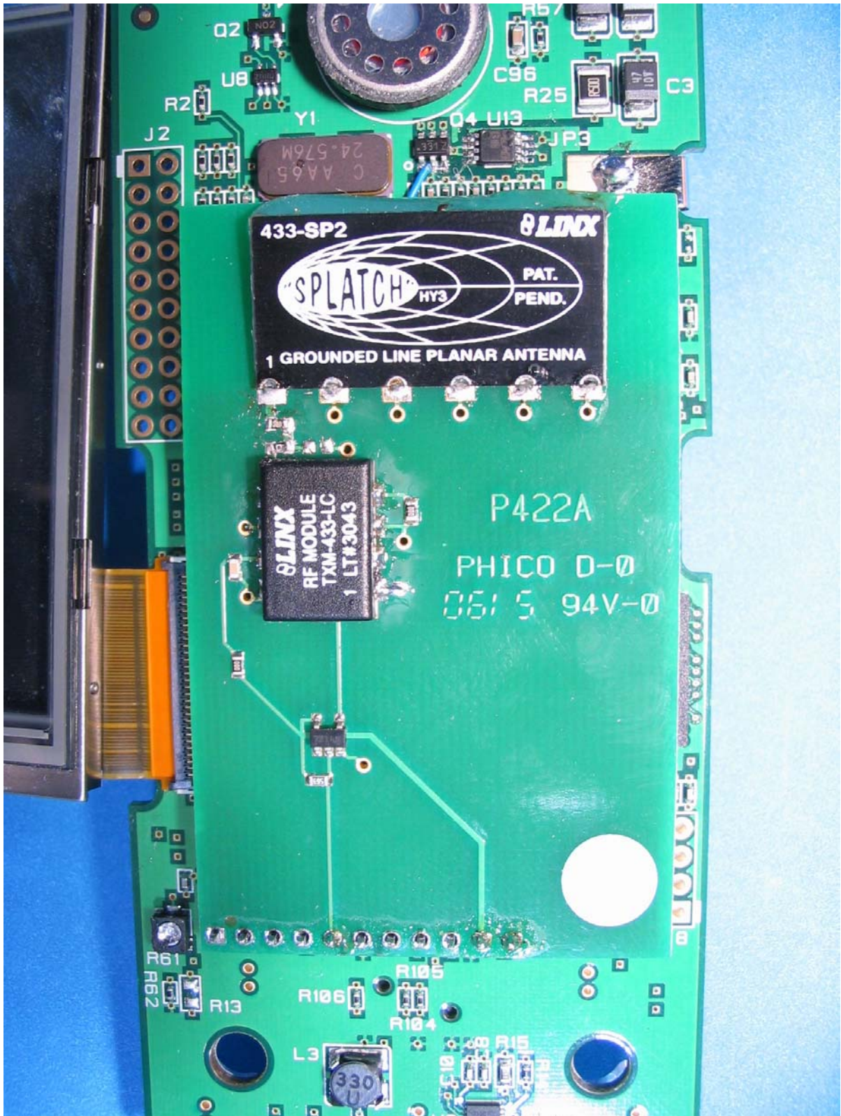
Figure 5: Daughter Board Bottom
