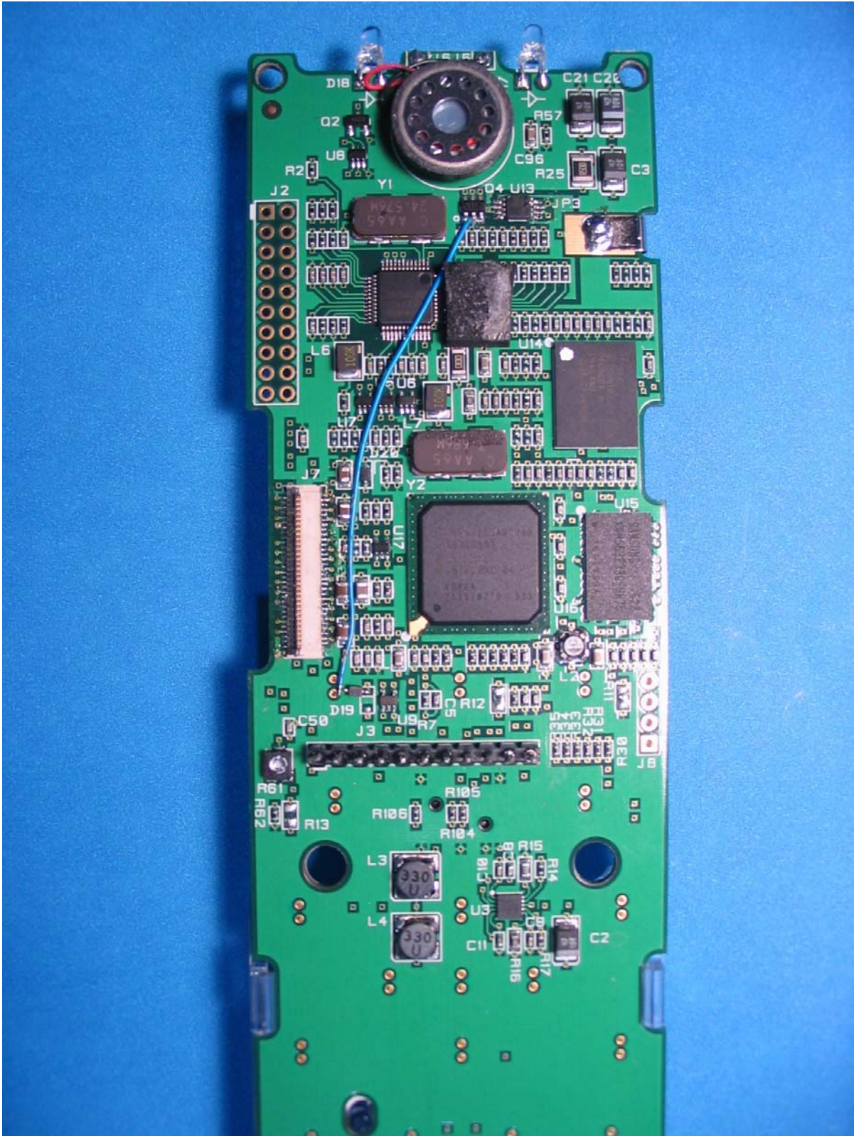
Figure 4: Main Board Under Daughter Board
