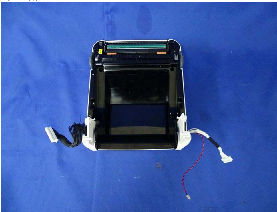
(28) EUT Photo
