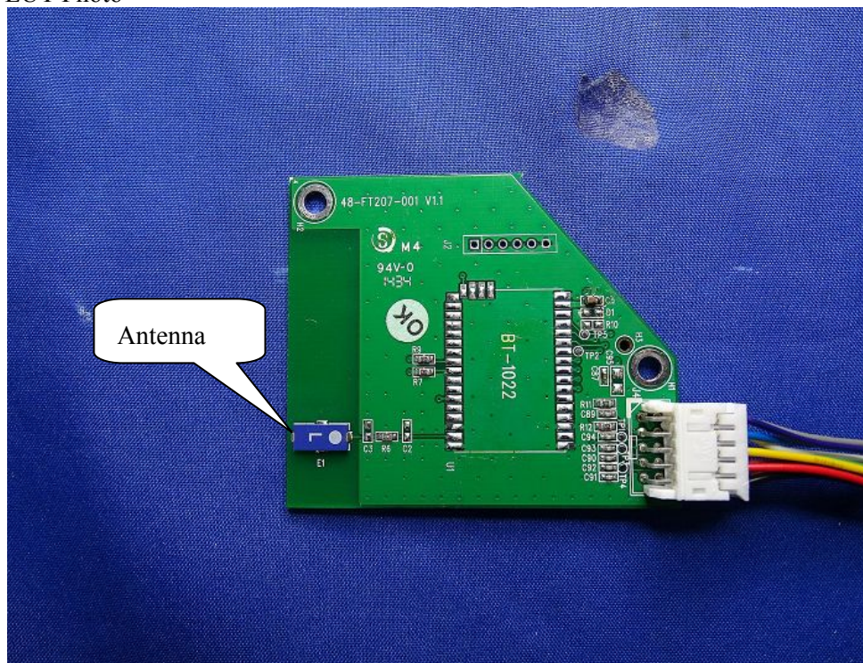
(23) EUT Photo
