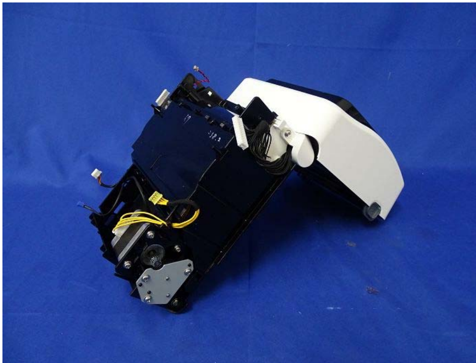
(26) EUT Photo
