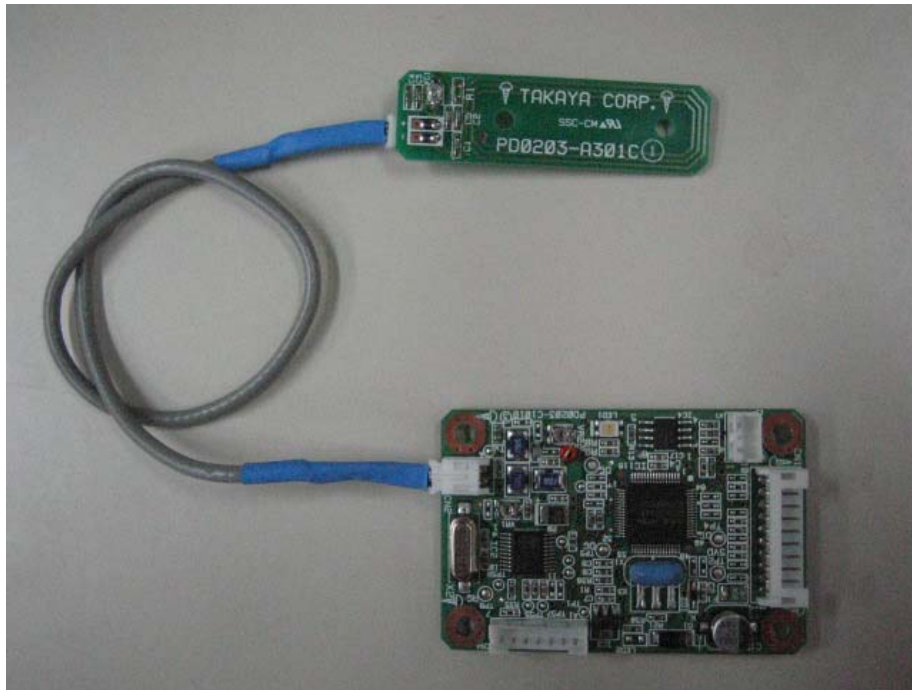
RFID Reader/Writer Module with Antenna
