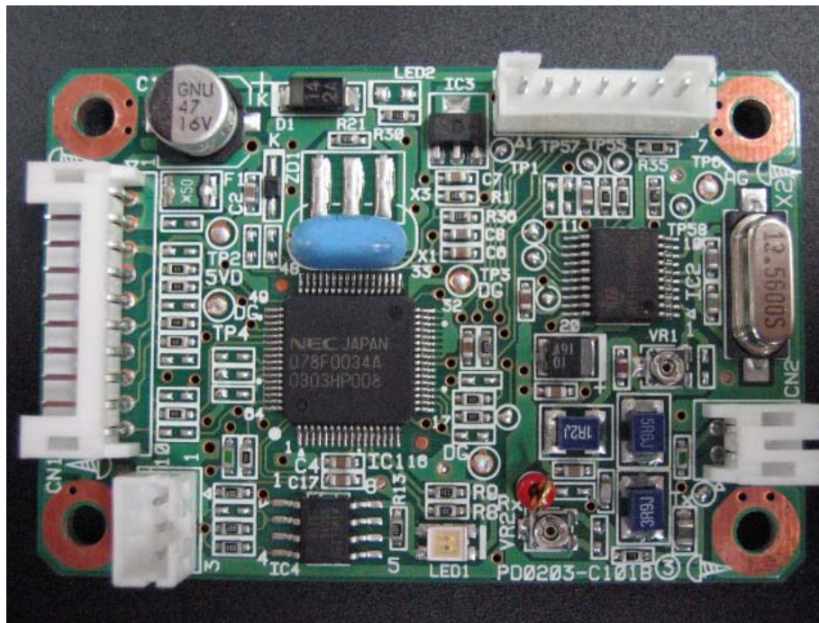
RFID Reader/ Writer Module – Front
