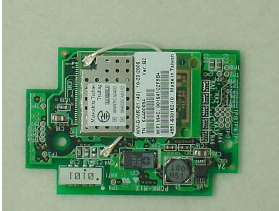
Front with Shield
