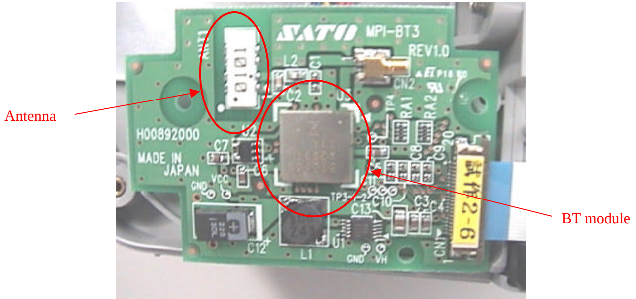
Inside Printer, Front View of PCB
