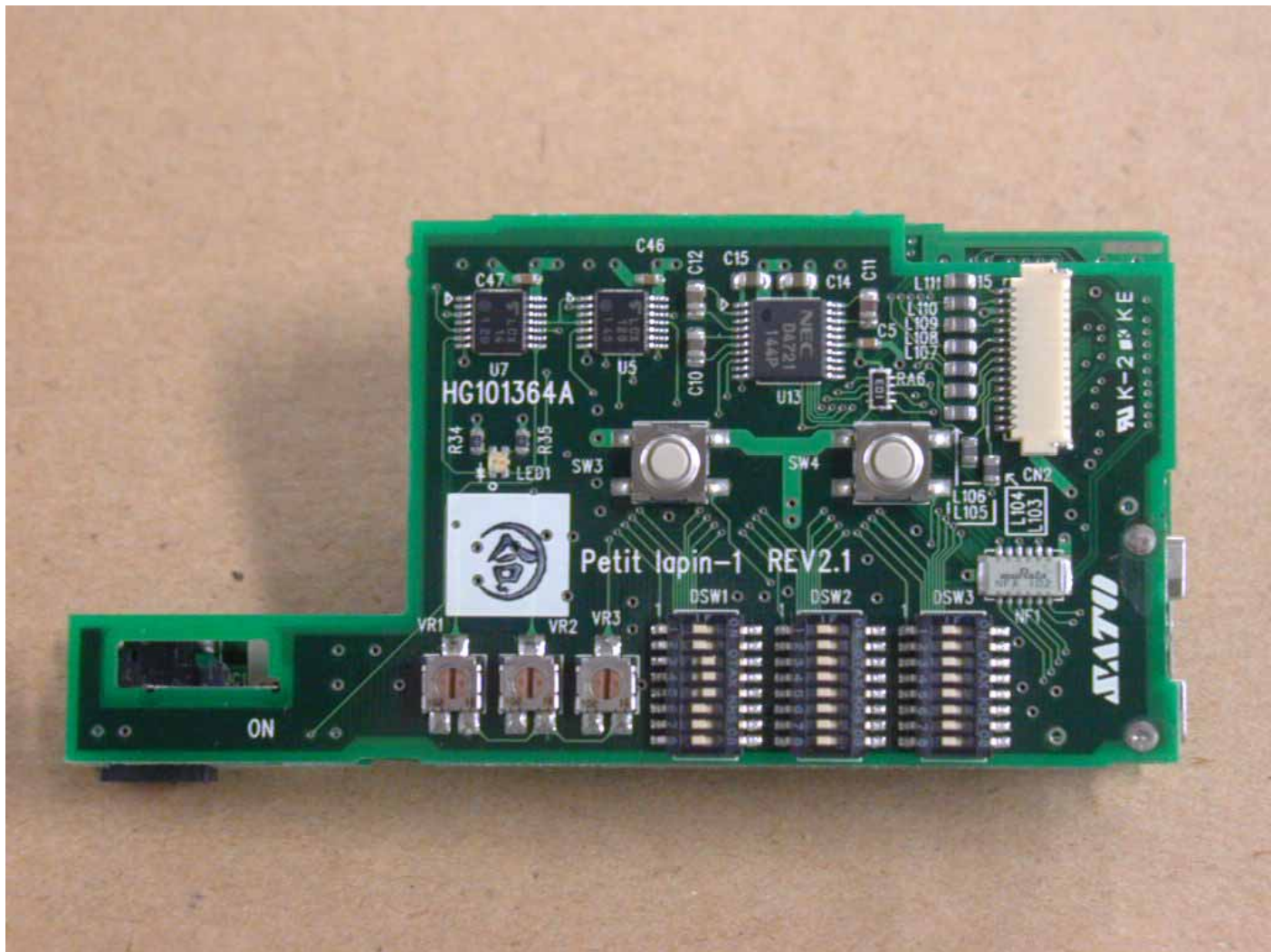
- Circuit Board 1(A side) -
