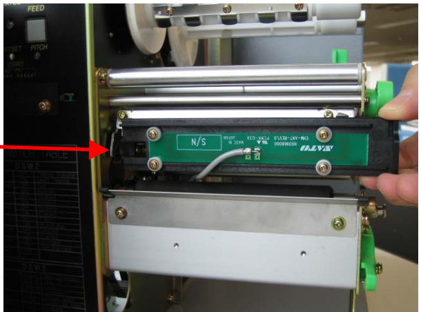
Antenna Position
