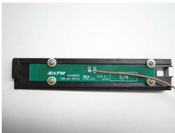
Antenna Holder
