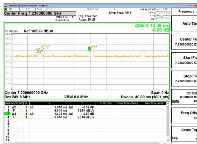
Radio 1 : The duty cycle of 2nd harmonics is 8%
