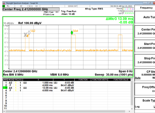
Radio 1 : The duty cycle of fundamental signal (2412MHz) is 8 %
