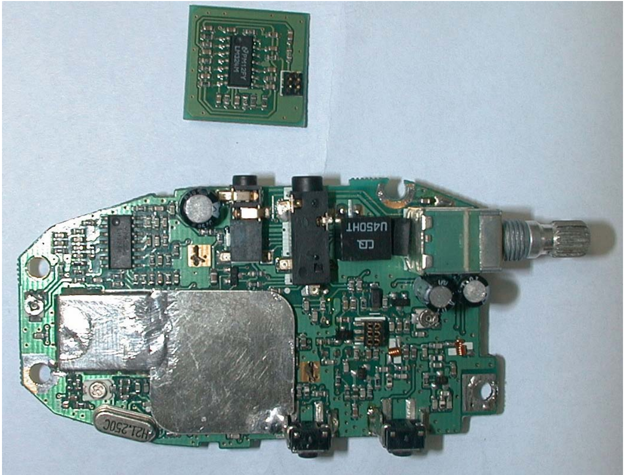
PCB Bottom w/shield
