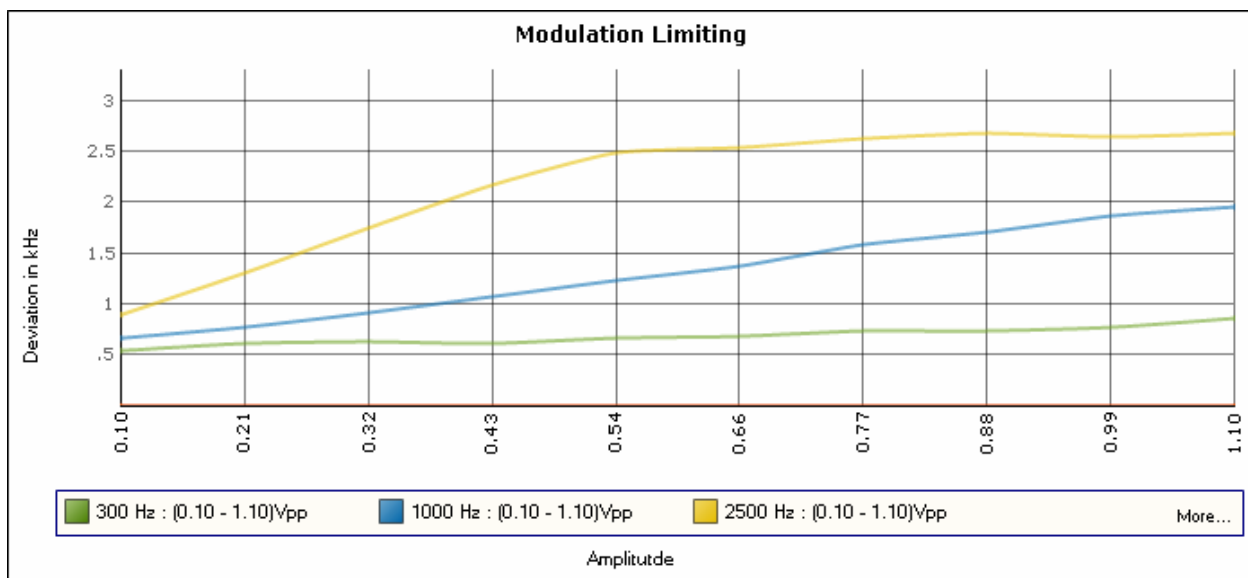
Modulation Limiting Plot (12.5 kHz)
