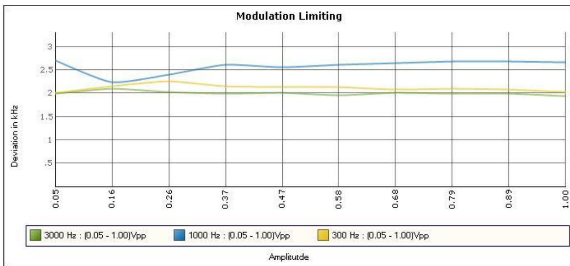
Modulation Limiting Plot (12.5 kHz)
