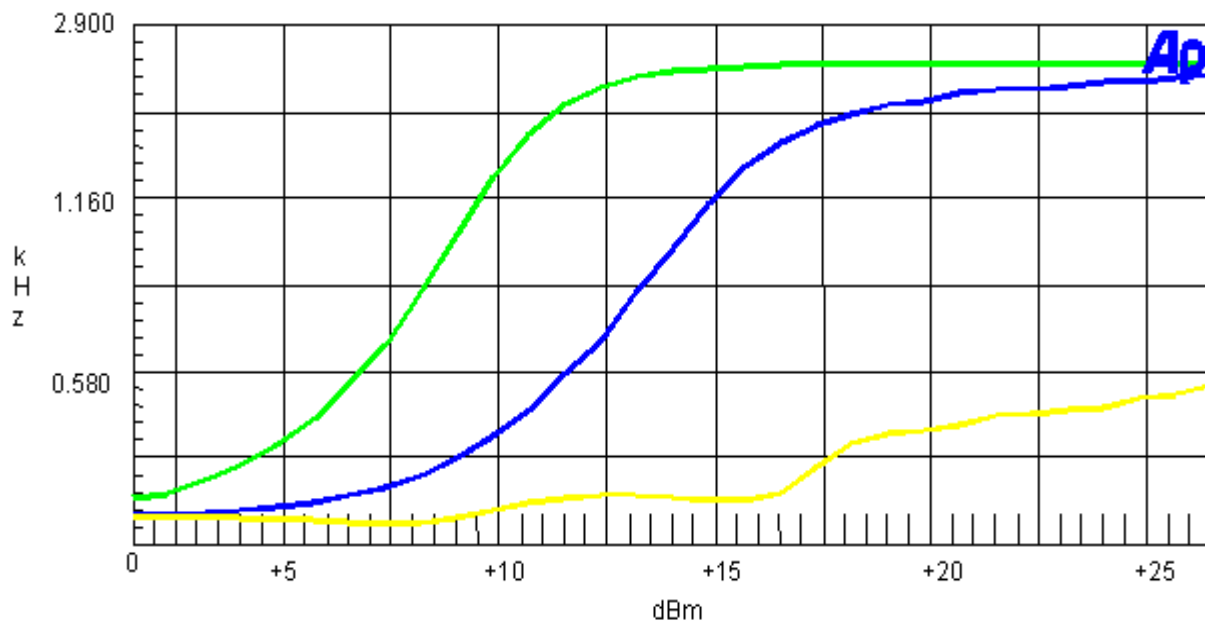
Modulation Limiting Plot 12.5kHz 2.5 KHz (Green), 1.0 KHz (Blue), and 300 Hz (Yellow)
