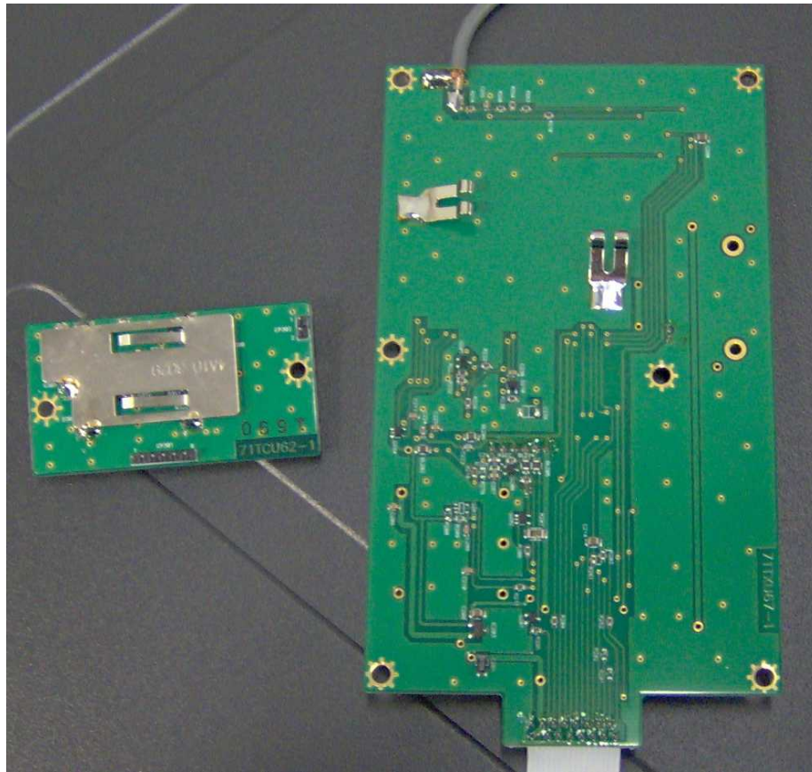
TX MODULE BOARDS BOTTOM
