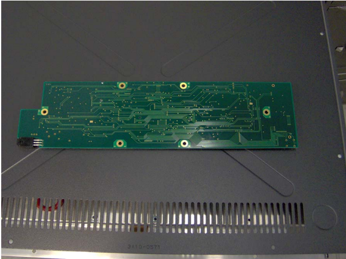
LOGIC PCB BOTTOM
