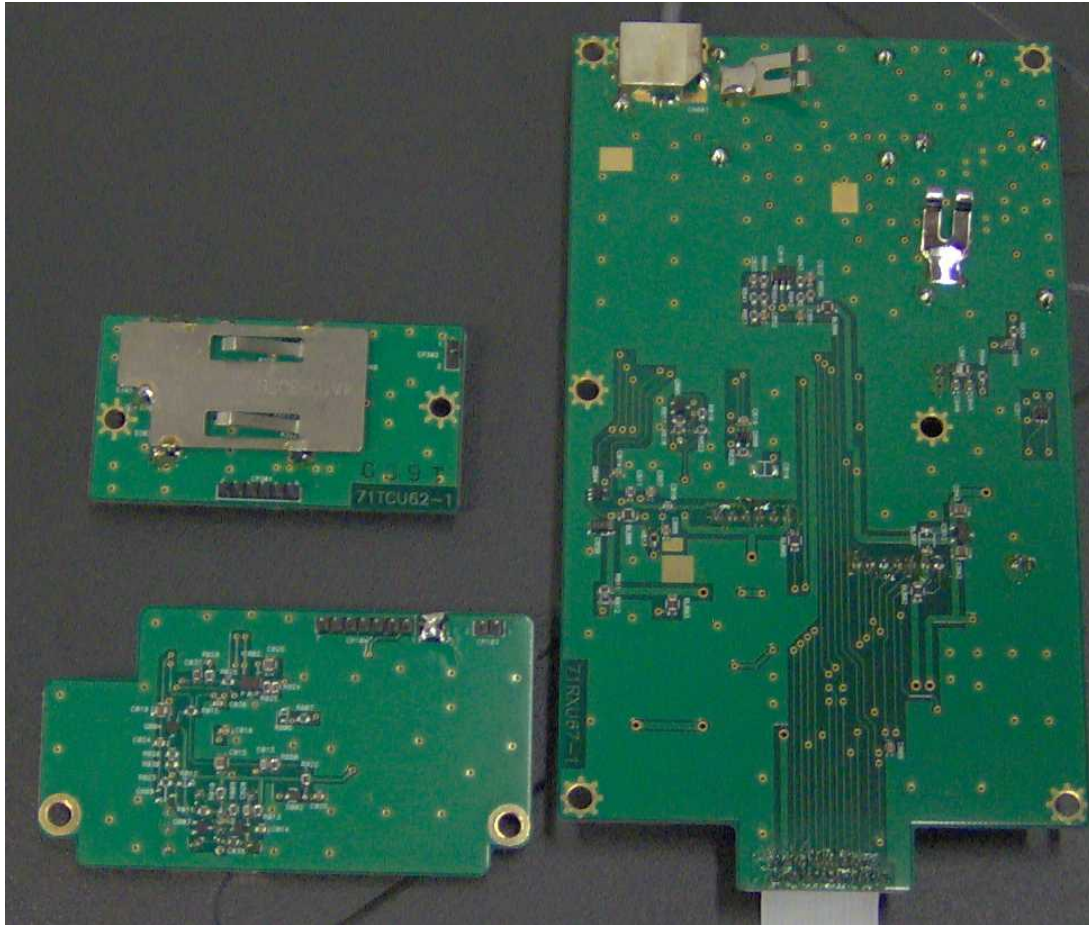
RX MODULE BOARDS BOTTOM
