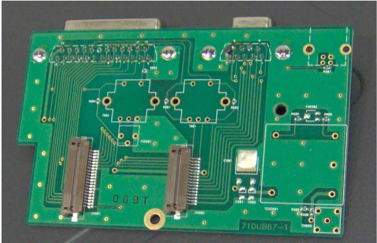
EXT OPTION PCB TOP
