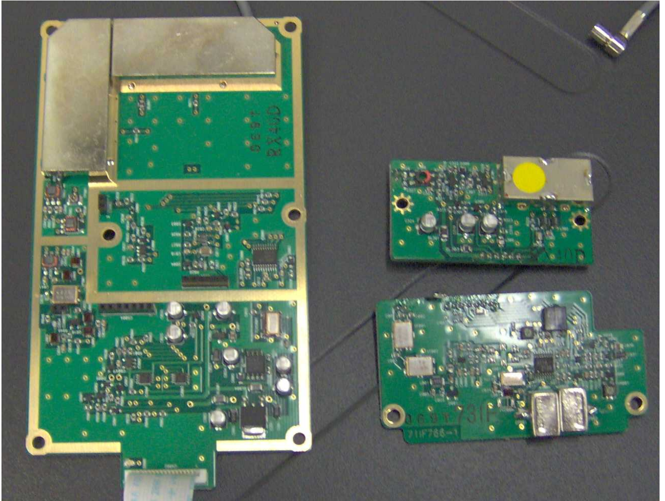
RX MODULE BOARDS TOP
