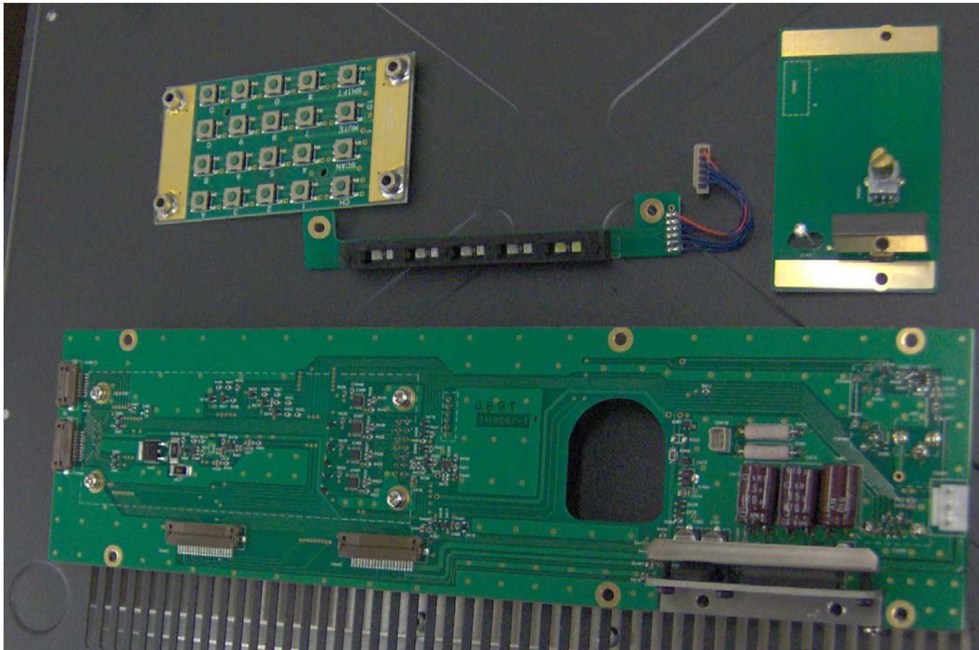
FRONT PANEL BOARDS TOP
