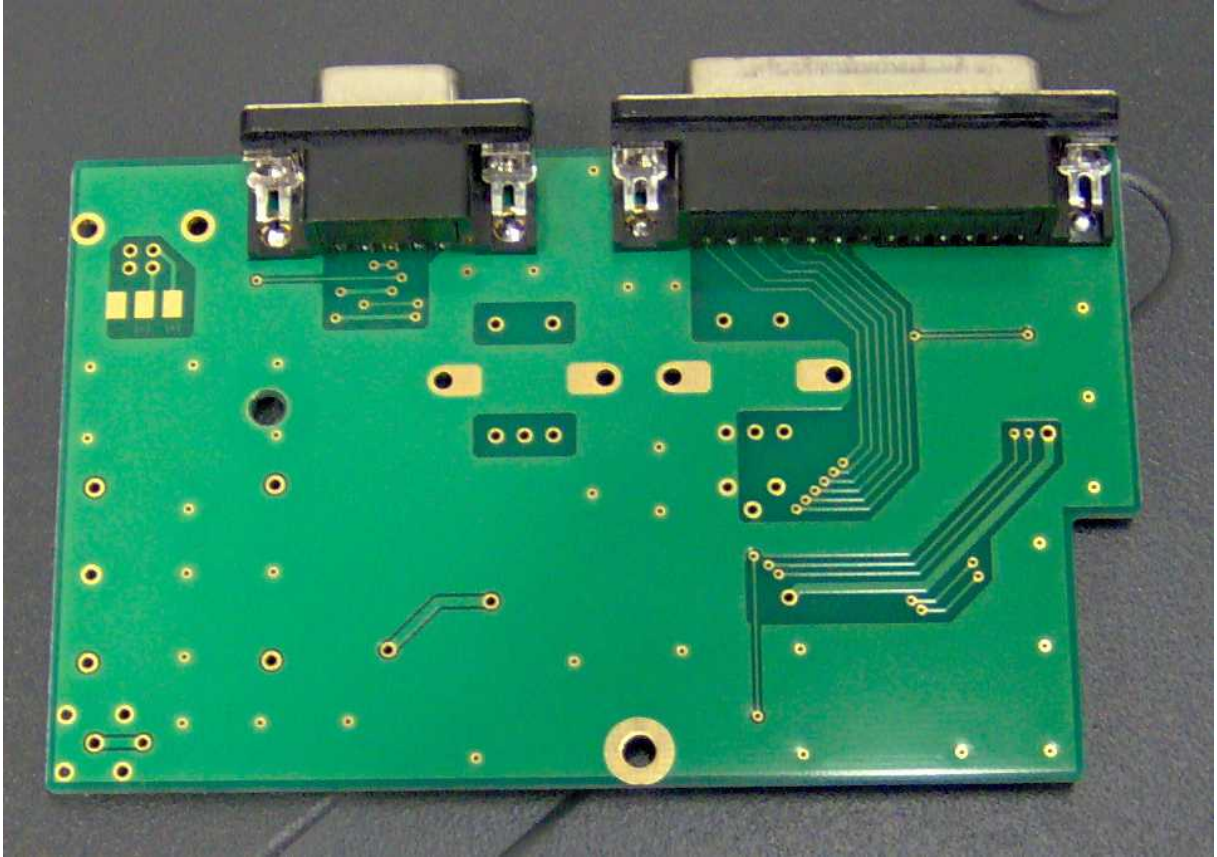
EXT OPTION PCB BOTTOM
