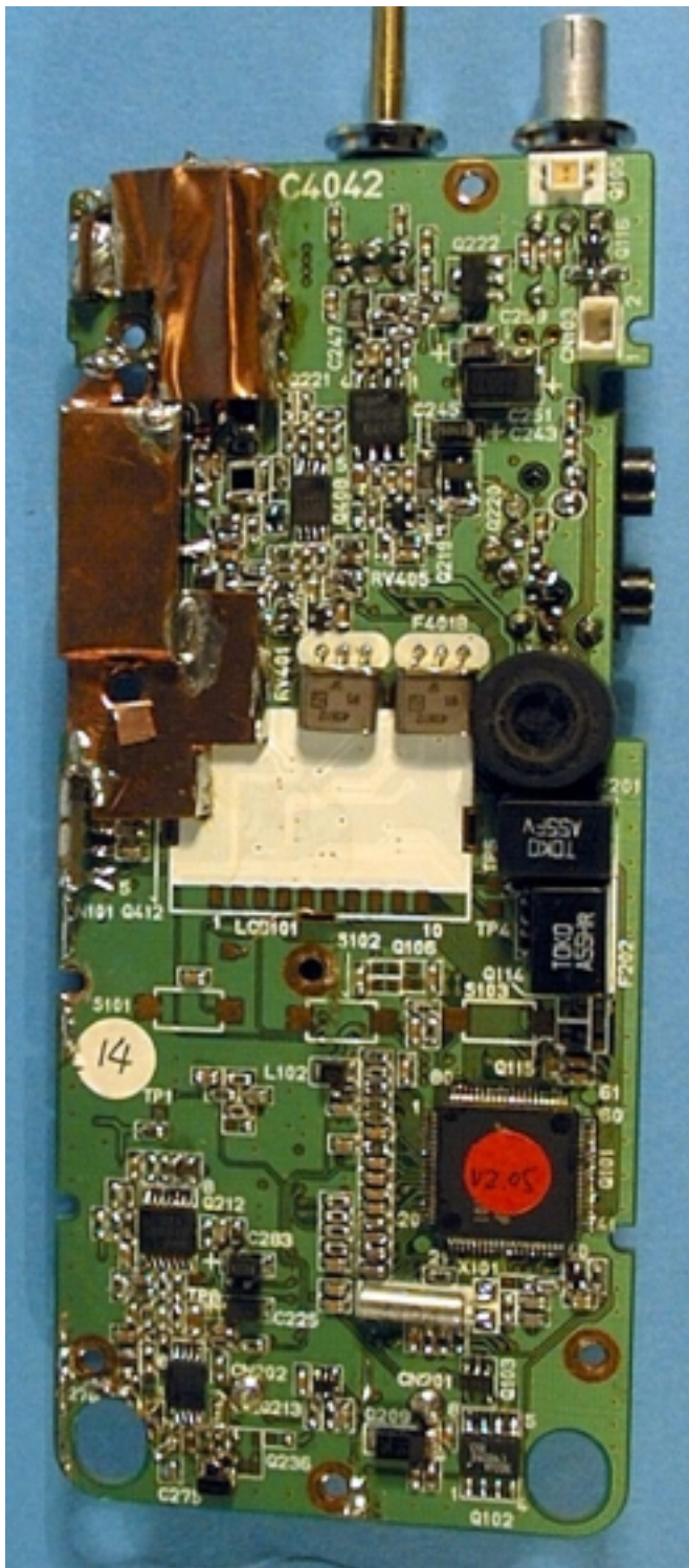
Main Board Top w/Shield
