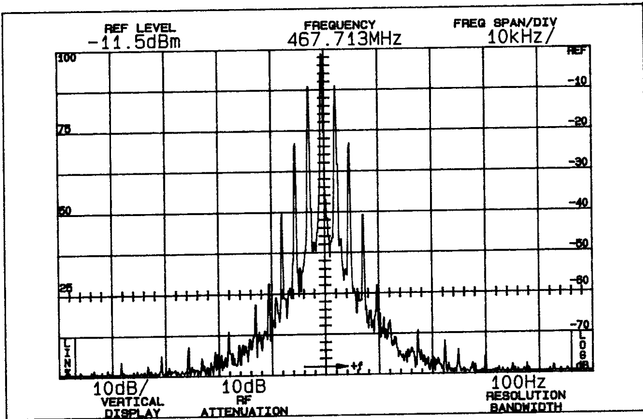
FIGURE 4 OCCUPIED BANDWIDTH
