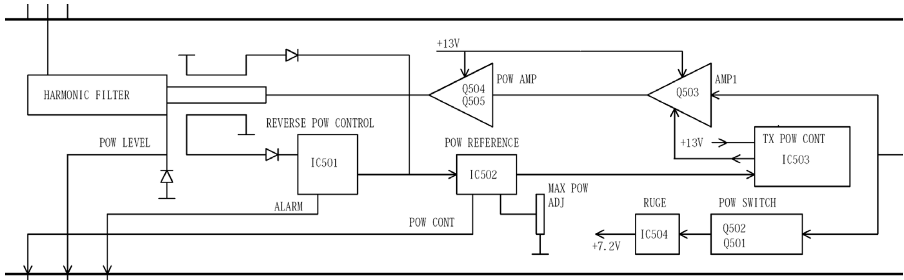
PA section block diagram for 71-0110 (A,B, or C)
