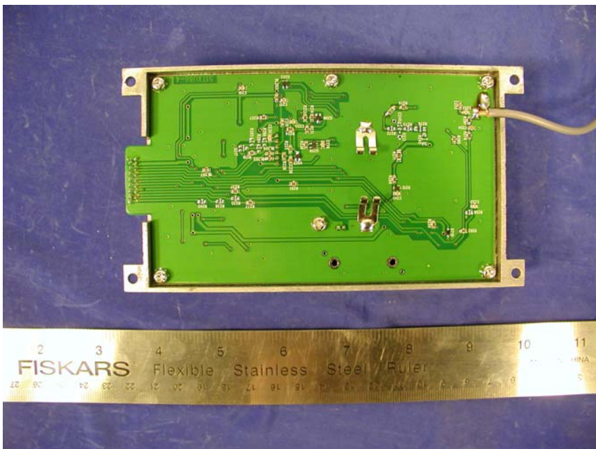
EUT – Transmitter Solder View
