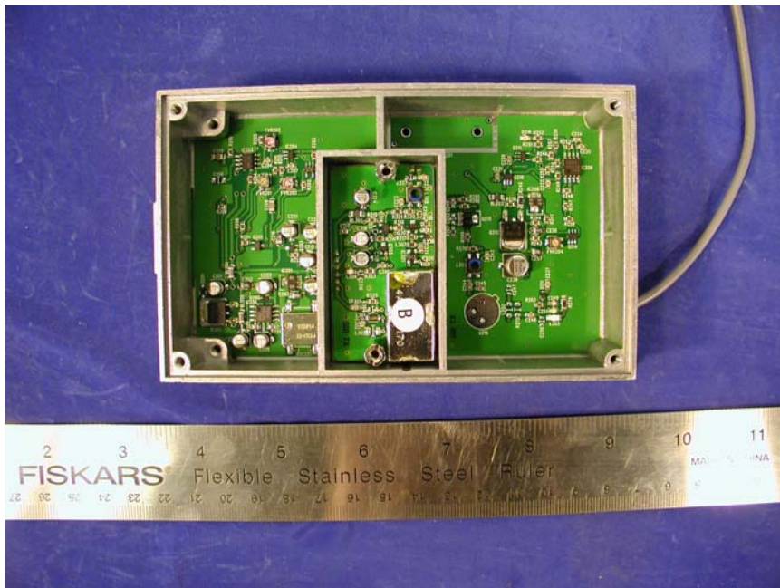
EUT - Transmitter Component View
