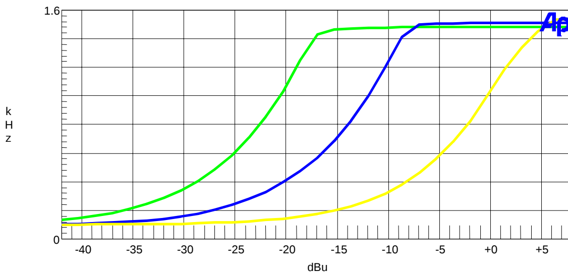
Modulation Limiting Plots Narrow Band: 2.5KHz (Green), 1.0KHz (Blue), and 300Hz (Yellow)
