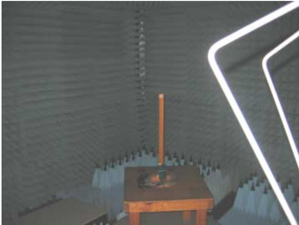
Photograph No.6 Radiated emissions measurement setup in the anechoic chamber with biconical antenna
