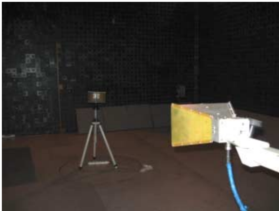
Photograph No.7 Setup for substitution measurements of spurious emissions in the anechoic chamber
