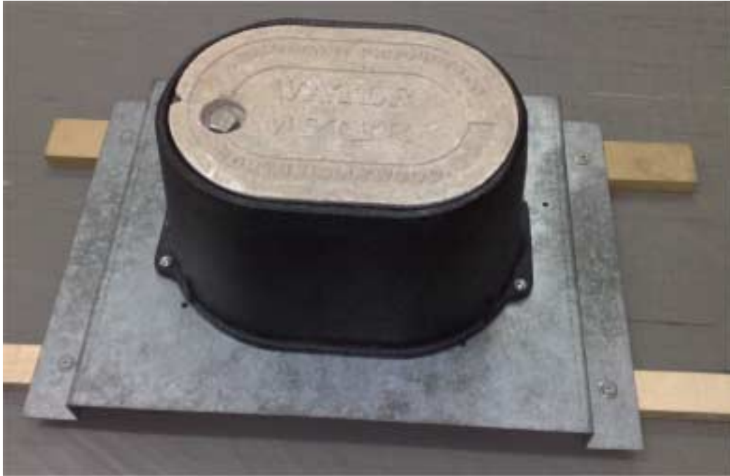
Photograph No.1 Typical water meter installation - Galaxy Pit2 transmitter inside metal pit with composite lid (cover)
