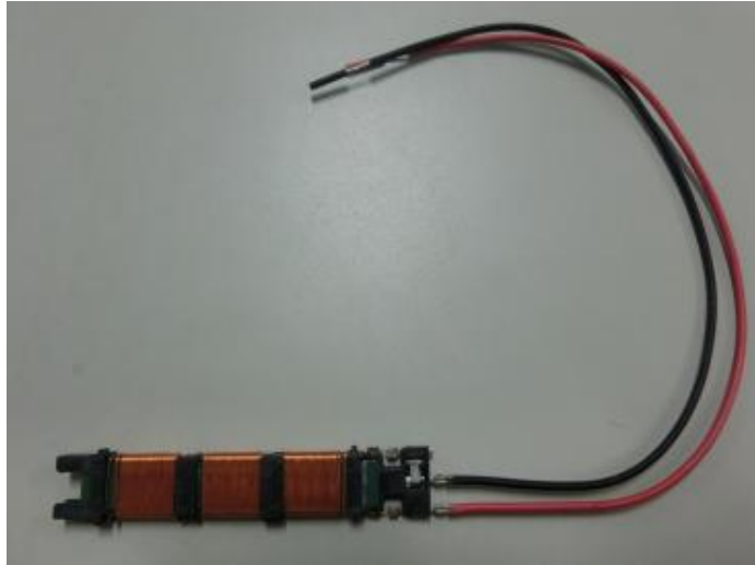
Ferrite coil antenna (Internal)
