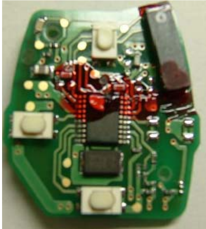
PWB Side A
