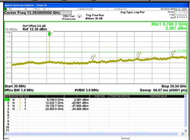
W58_11n20_Lower_Conducted Spurious
