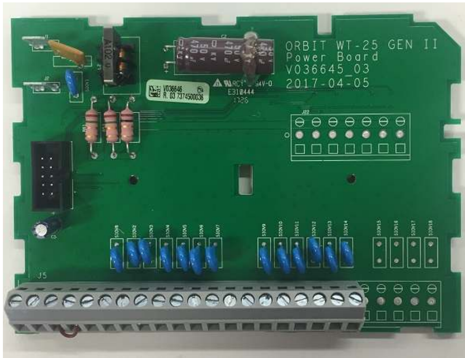
Top photo - Front side of power board Bottom photo - Back side of power board
