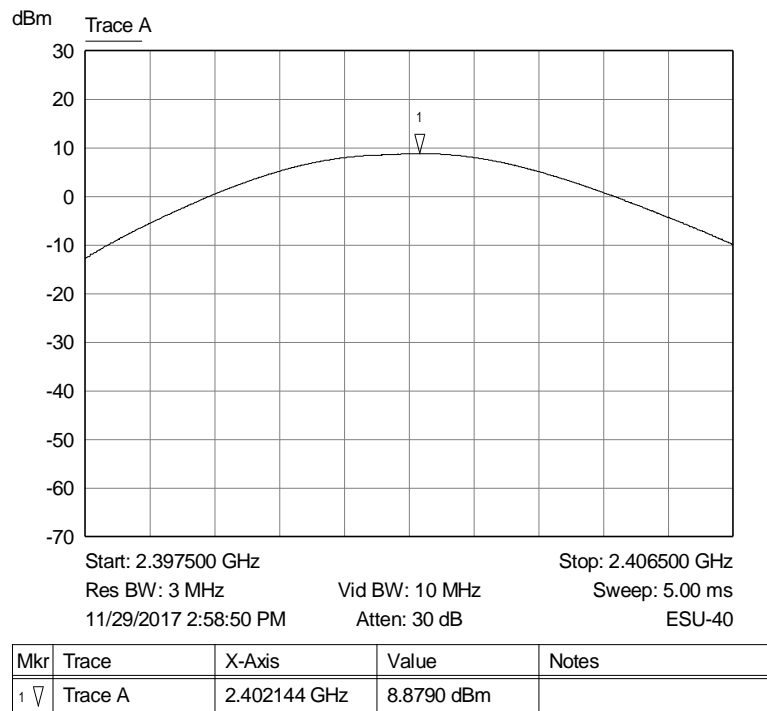
Graph 49: Lowest Channel Output Power Plot
