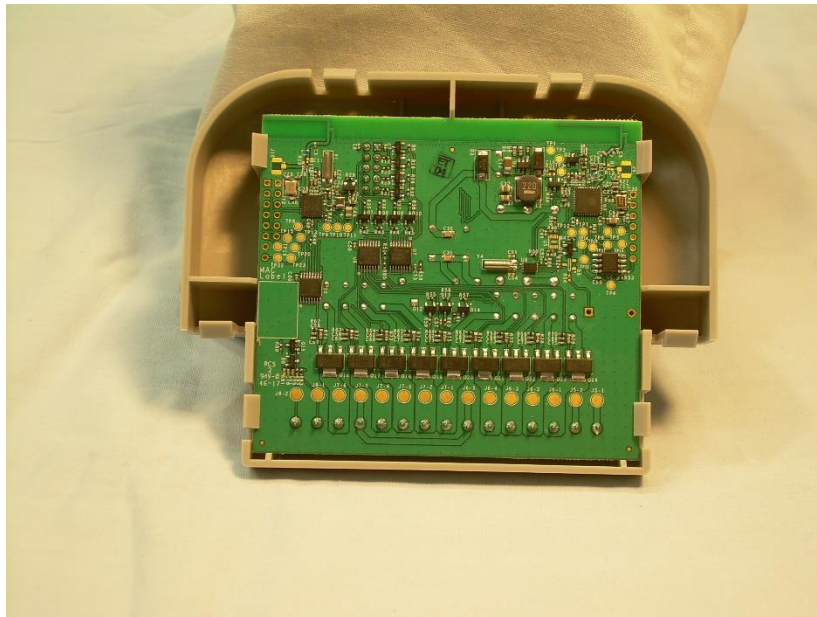
Photograph 13 – View of the PCB in the Housing
