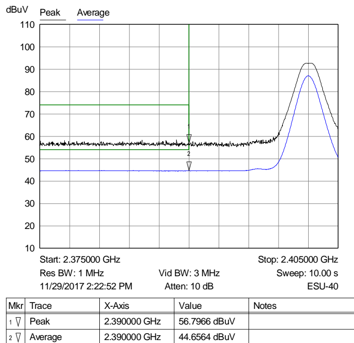
Graph 55: Radiated Lower Band Edge Plot – Horizontal Polarity
