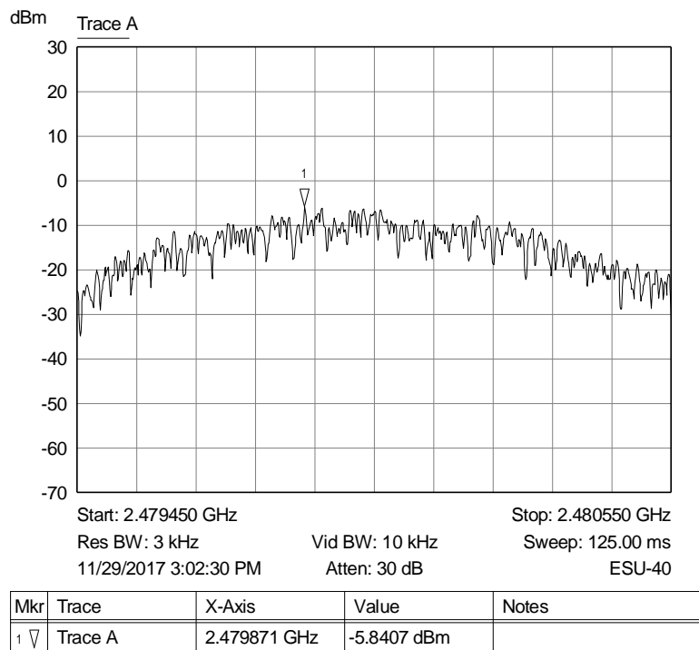
Graph 60: Highest Channel Output 3 kHz PSD Plot
