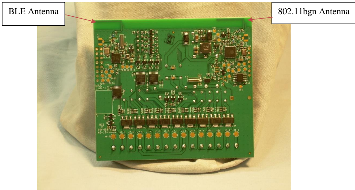
Photograph 15 – Back View of the PCB
