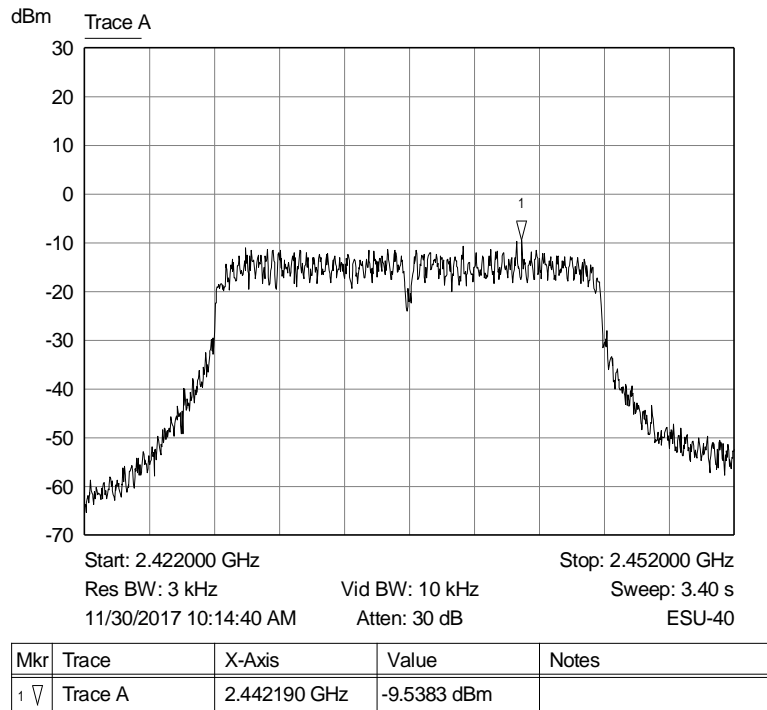
Graph 44: Middle Channel 3 kHz PSD Plot
