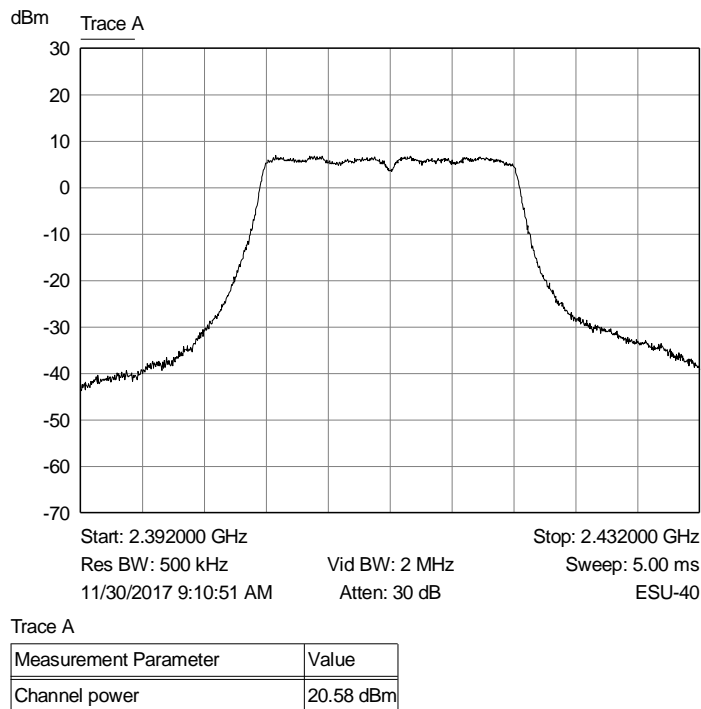
Graph 19: Lowest Channel Output Power Plot
