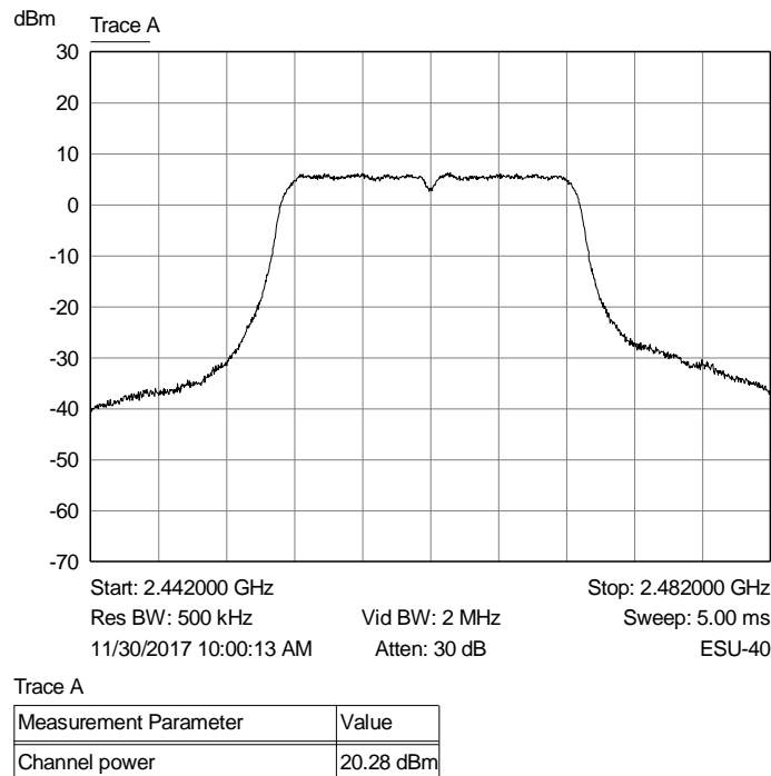
Graph 36: Highest Channel Output Power Plot
