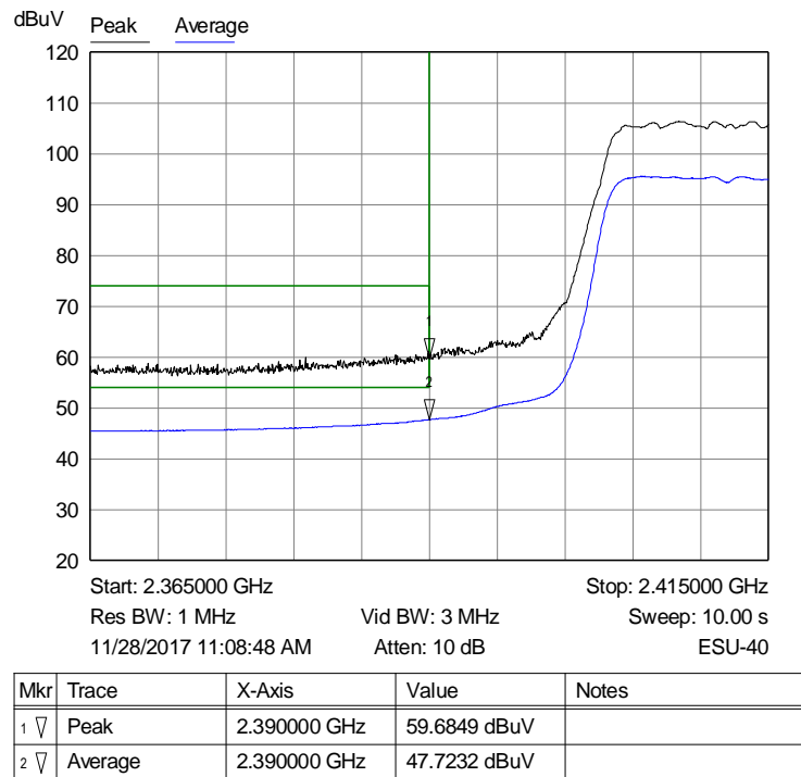
Graph 39: Radiated Lower Band Edge Plot – Vertical Polarity
