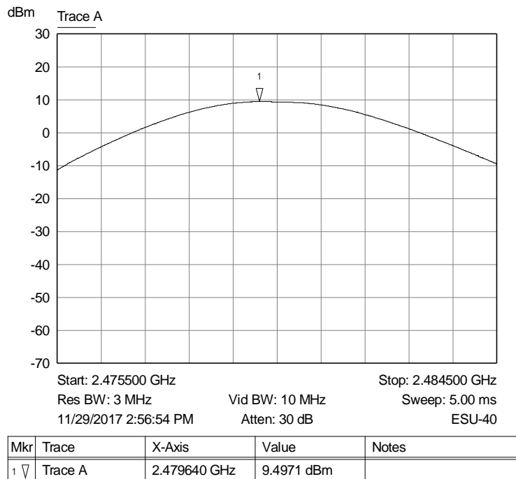
Graph 51: Highest Channel Output Power Plot
