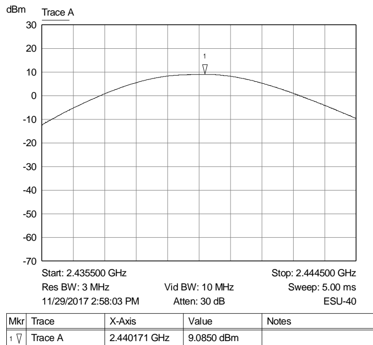
Graph 50: Middle Channel Output Power
