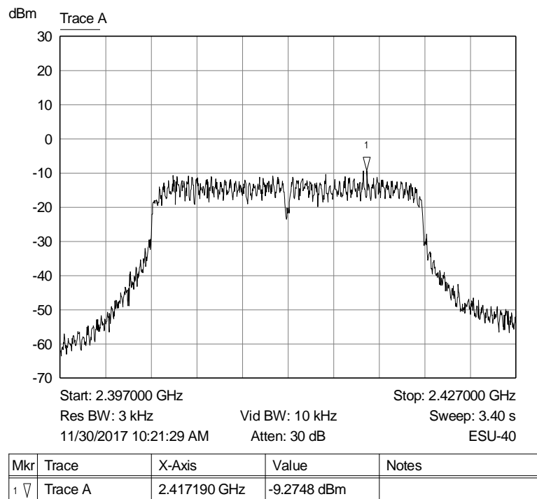
Graph 43: Lowest Channel 3 kHz PSD Plot
