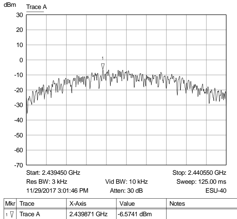
Graph 59: Middle Channel 3 kHz PSD Plot
