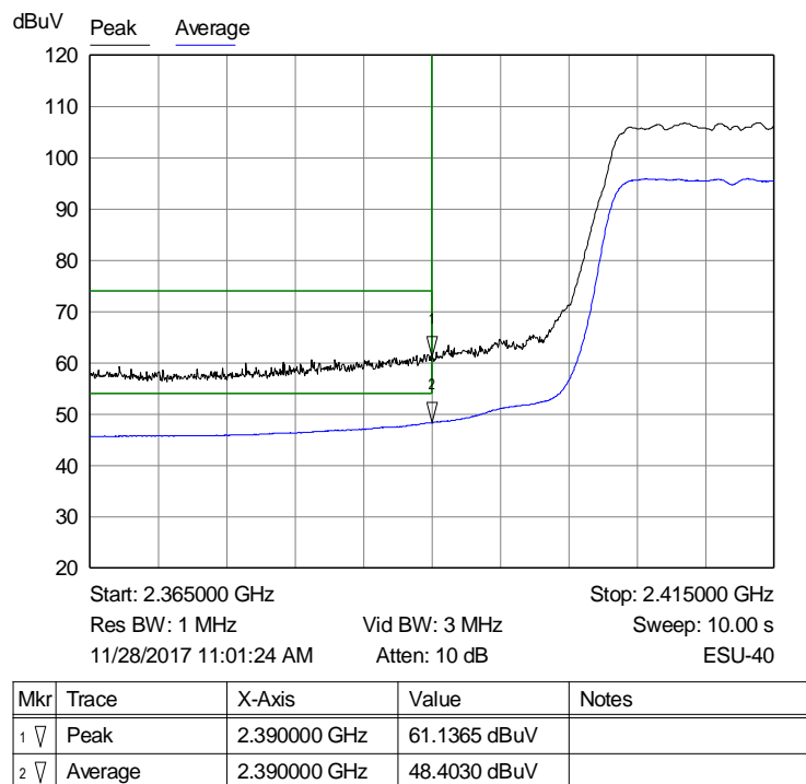
Graph 40: Radiated Lower Band Edge Plot – Horizontal Polarity
