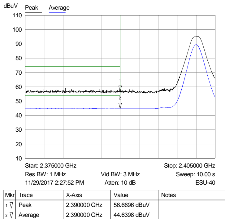
Graph 54: Radiated Lower Band Edge Plot – Vertical Polarity
