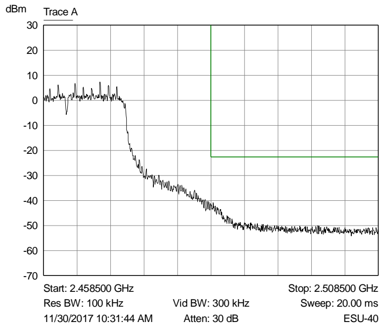
Graph 38: Upper Band Edge Plot
