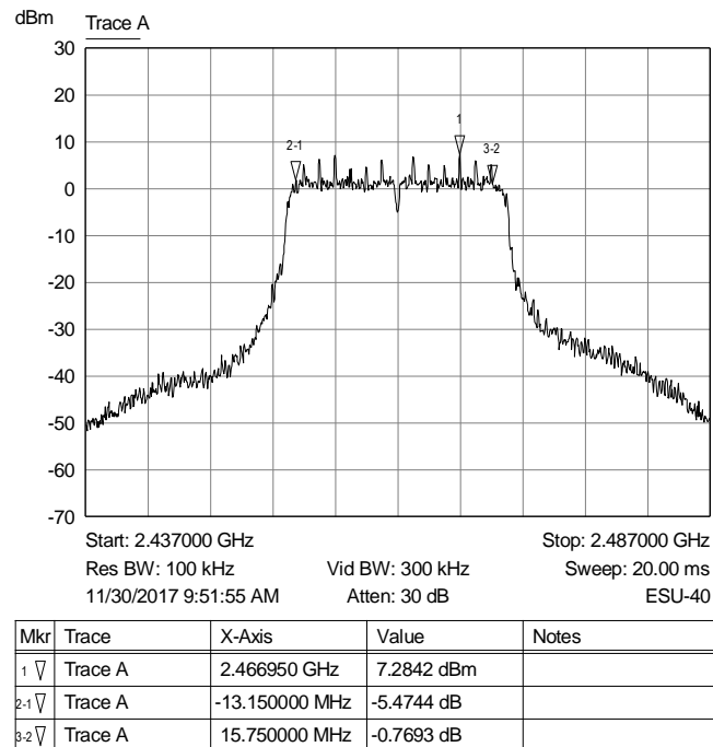
Graph 33: Highest Channel Bandwidth
