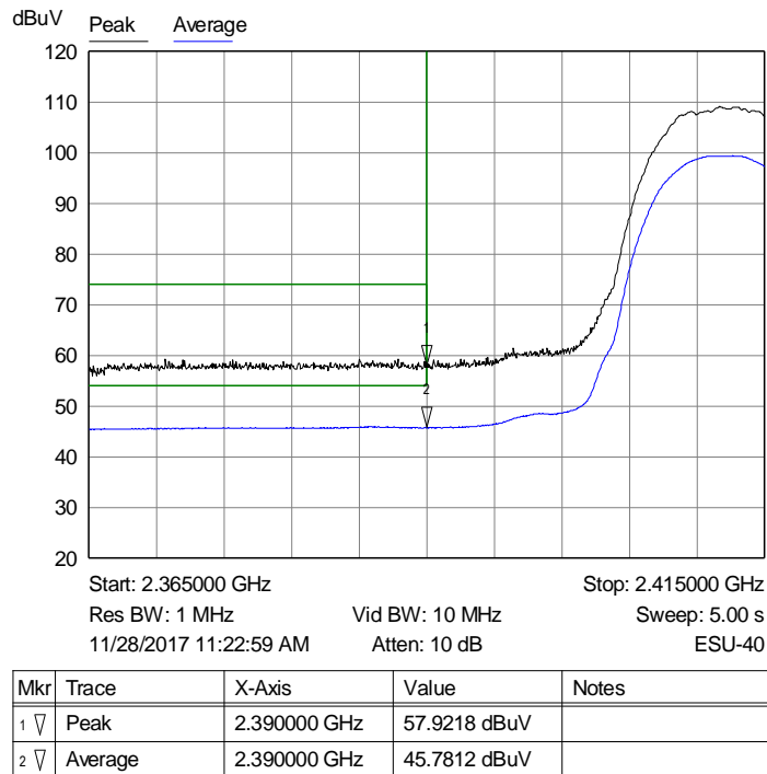
Graph 9: Radiated Lower Band Edge Plot – Vertical Polarity
