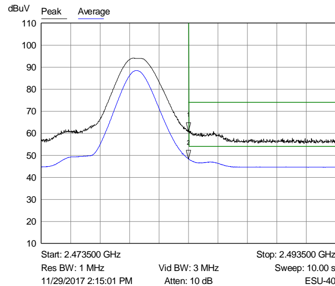
Graph 56: Radiated Upper Band Edge Plot – Vertical Polarity
