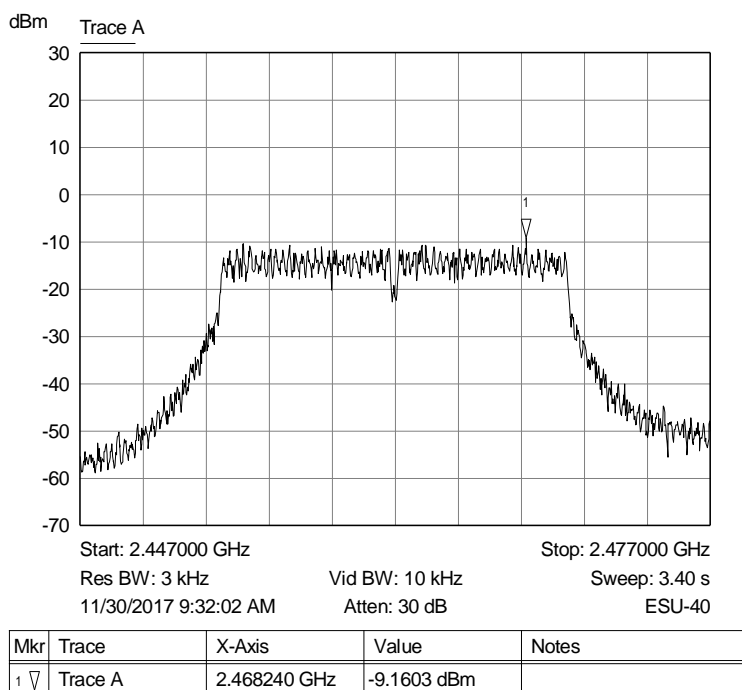
Graph 30: Highest Channel Output 3 kHz PSD Plot
