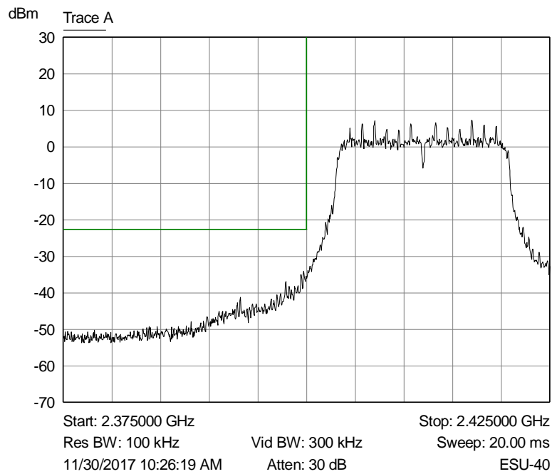
Graph 37: Lower Band Edge Plot
