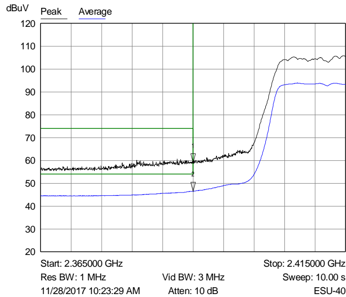
Graph 24: Radiated Lower Band Edge Plot – Vertical Polarity
