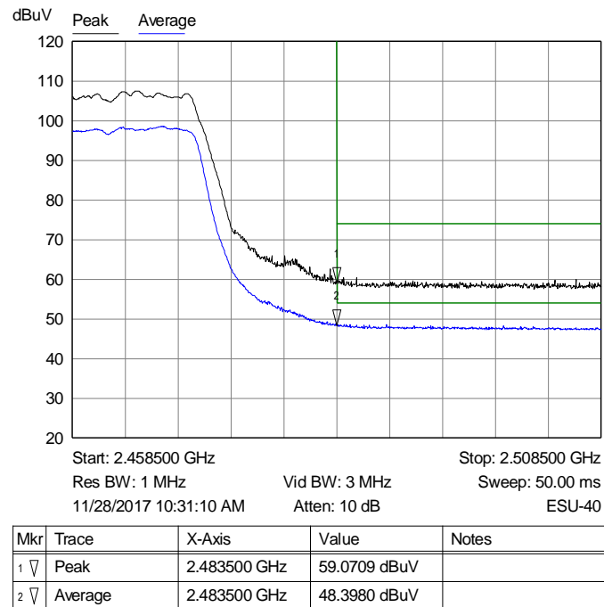
Graph 27: Radiated Upper Band Edge Plot – Horizontal Polarity
