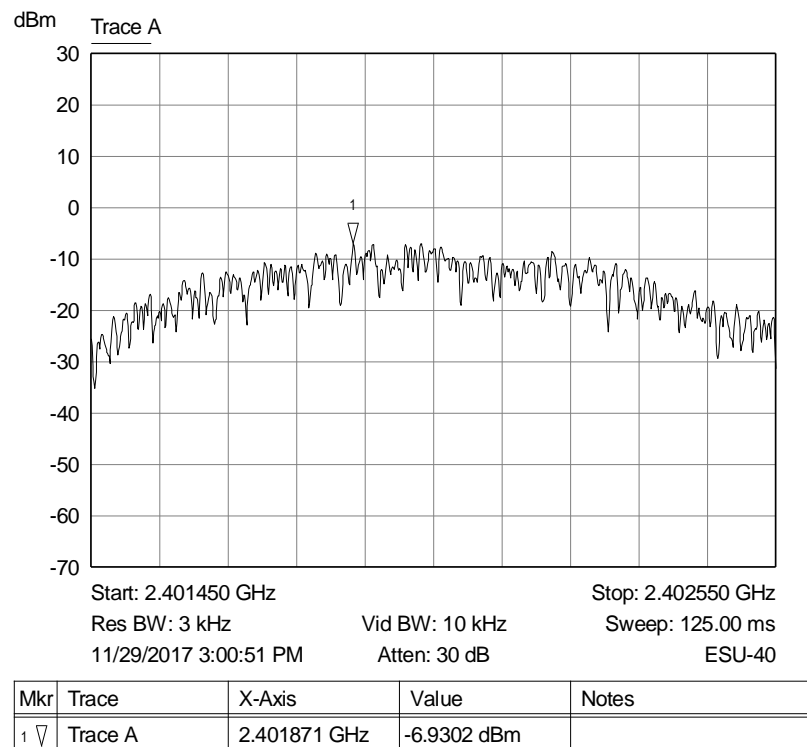
Graph 58: Lowest Channel 3 kHz PSD Plot
