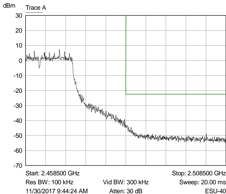
Graph 23: Upper Band Edge Plot
