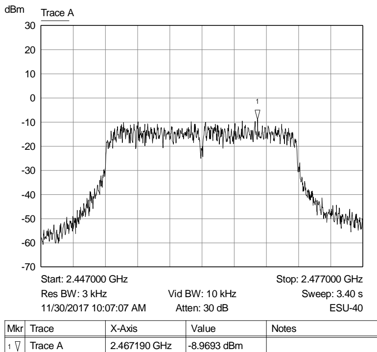
Graph 45: Highest Channel Output 3 kHz PSD Plot
