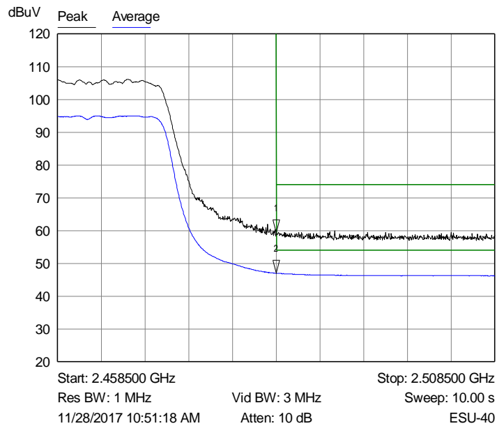
Graph 41: Radiated Upper Band Edge Plot – Vertical Polarity
