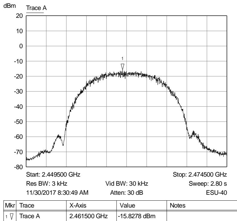
Graph 15: Highest Channel Output 3 kHz PSD Plot
