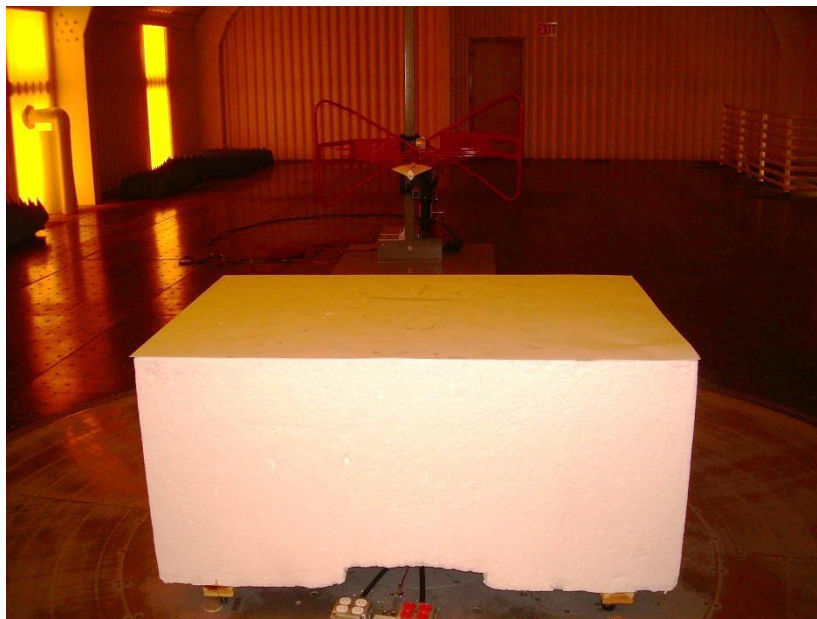
Photograph 18: Test Setup for Emission from 30 MHz to 1000 MHz
