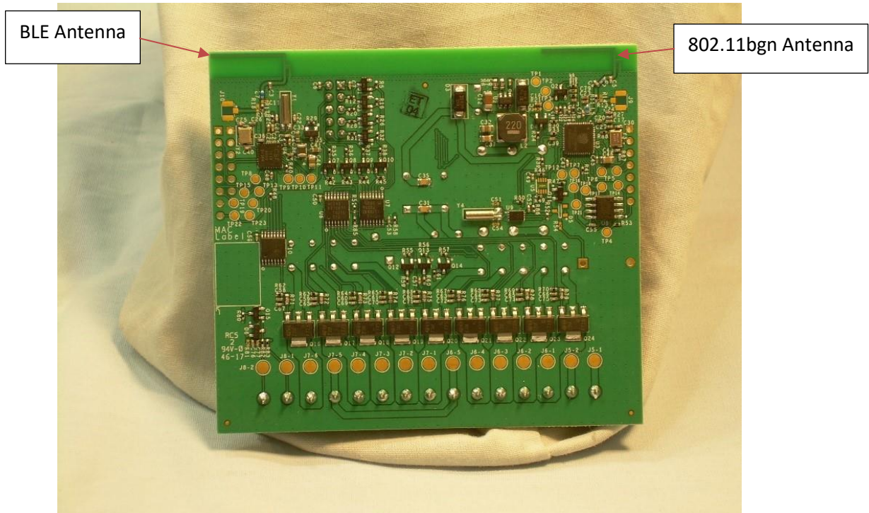
Photograph 3 – Back View of the EUT PCB
