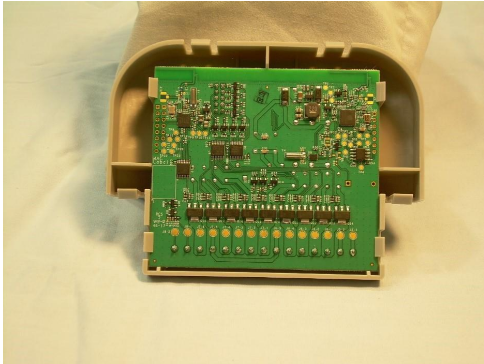
Photograph 1 – View of the PCB in the EUT Housing
