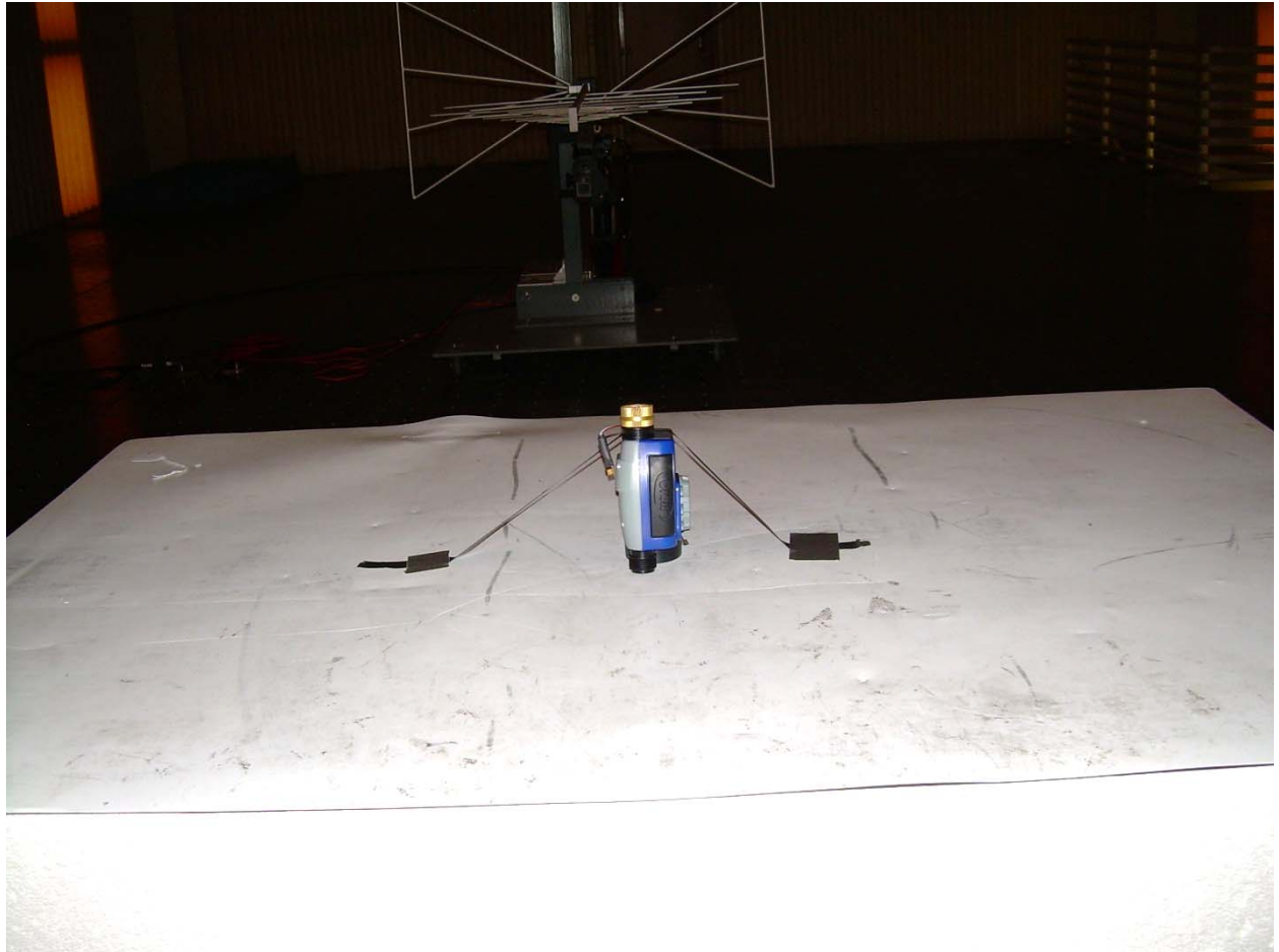
View Radiated Test Setup – Vertical Placement
