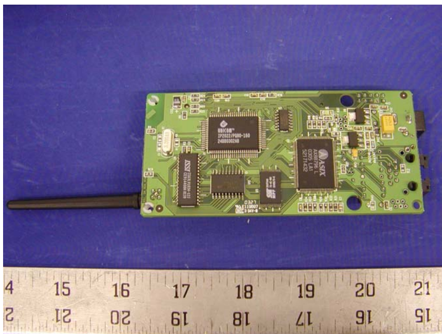
EUT – Component View with Antenna
