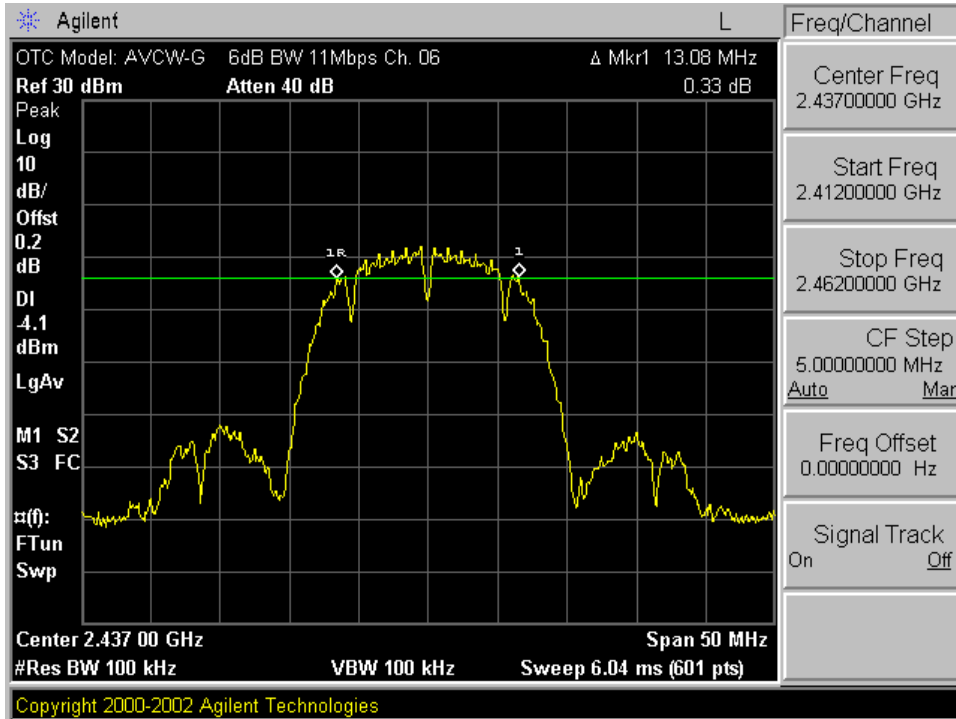
Plot A-2. 6dB 11Mbps Bandwidth Plot – Ch. 06
