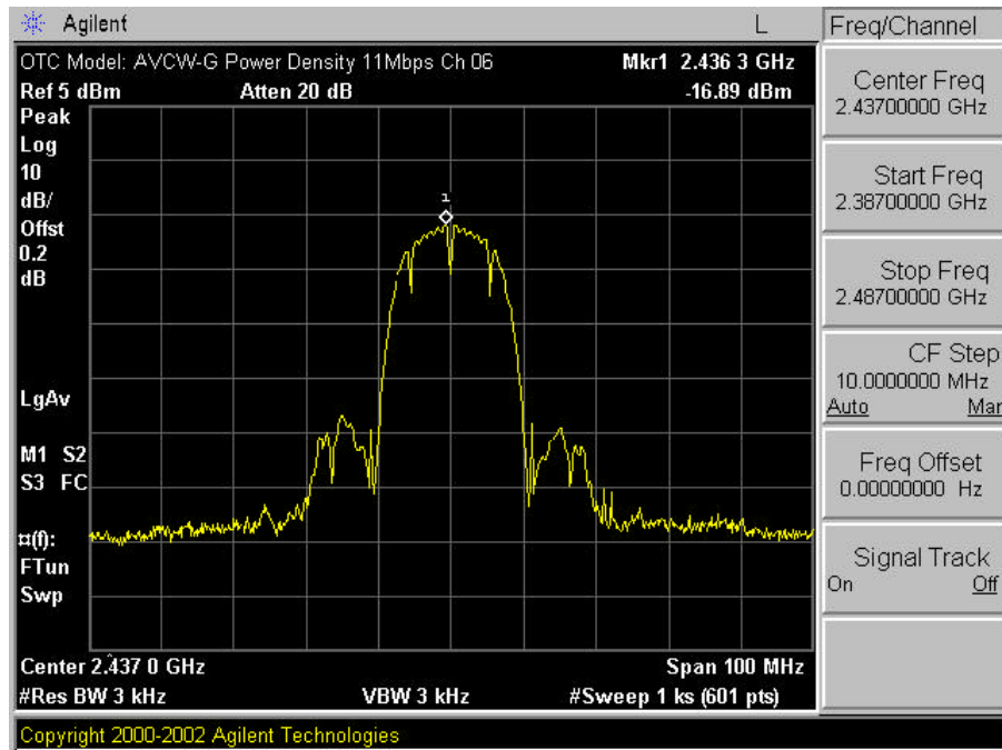
Plot A-8. Max. Power Density 11Mbps Plot – Ch. 06
