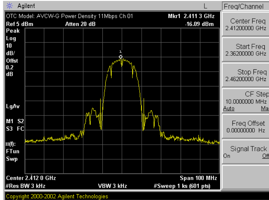
Plot A-7. Max. Power Density 11Mbps Plot – Ch. 01
