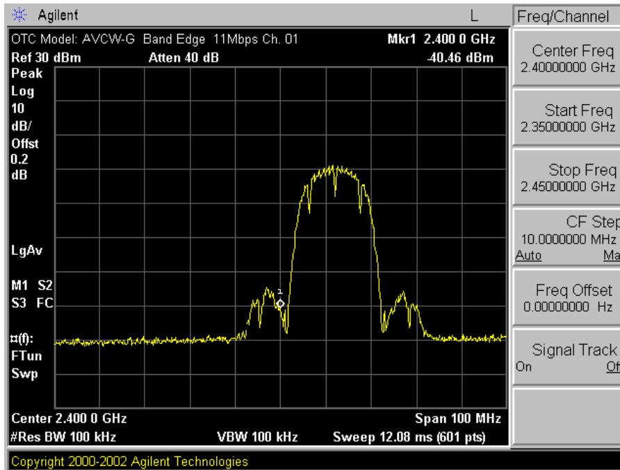
Plot A-10. Occupied Band Edge 11Mbps Plot – Ch. 01
