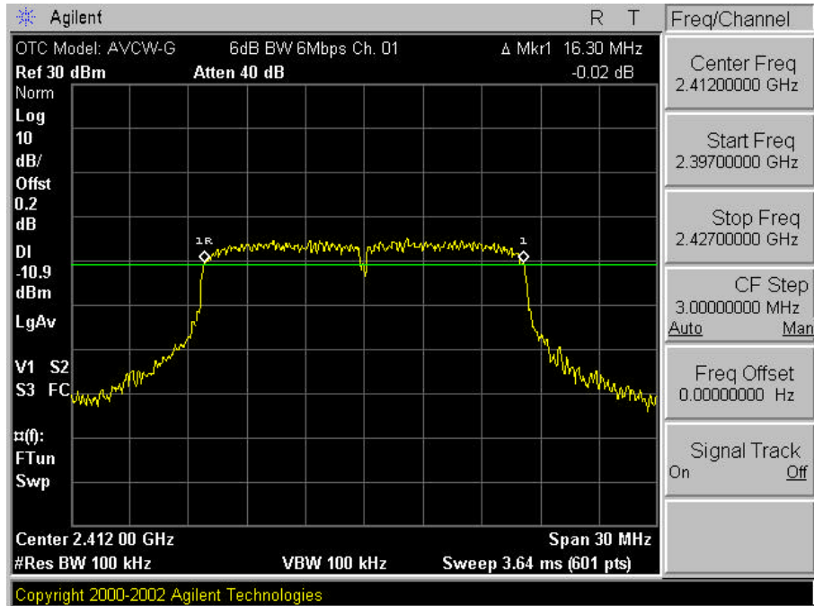
Plot A-1. 6dB 6Mbps Bandwidth Plot – Ch. 01
