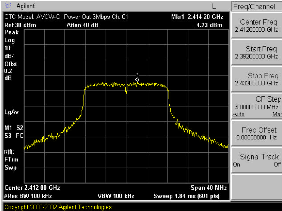
Plot A-4. Max. Output Power 6Mbps Plot – Ch. 01
