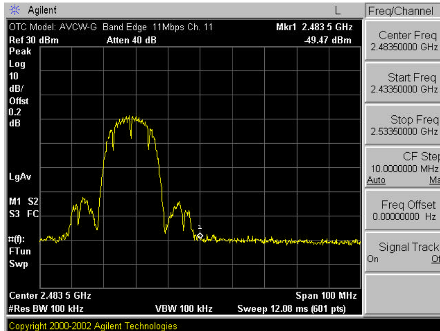
Plot A-11. Occupied Band Edge 11Mbps Plot – Ch. 11
