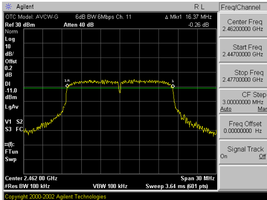
Plot A-3. 6dB 6Mbps Bandwidth Plot – Ch. 11
