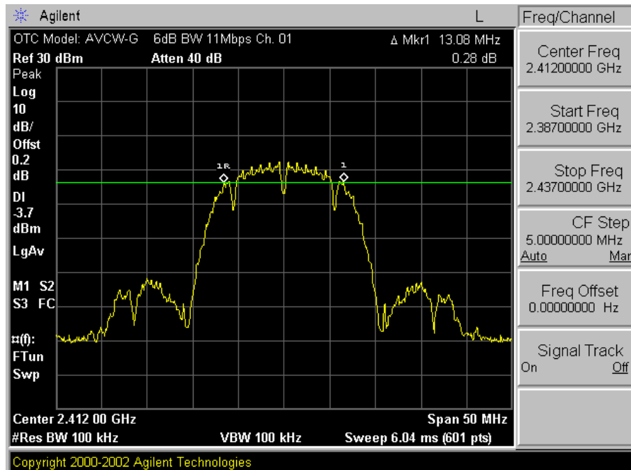
Plot A-1. 6dB 11Mbps Bandwidth Plot – Ch. 01
