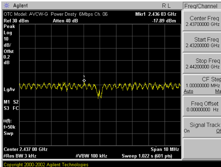
Plot A-8. Max. Power Density 6Mbps Plot – Ch. 06
