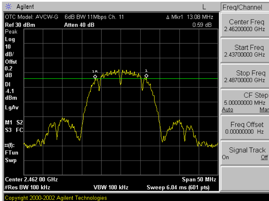
Plot A-3. 6dB 11Mbps Bandwidth Plot – Ch. 11
