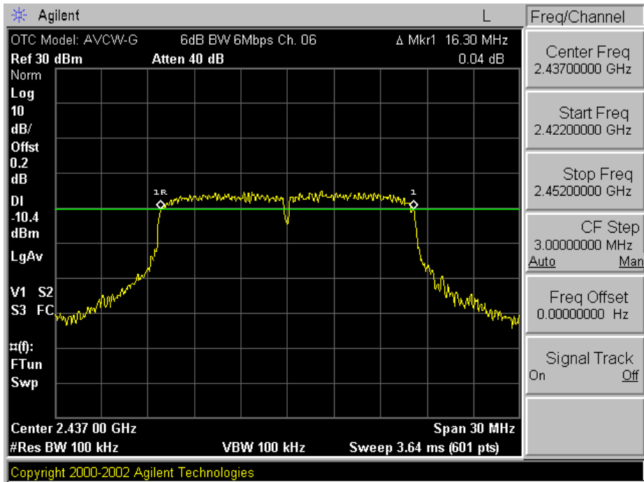
Plot A-2. 6dB 6Mbps Bandwidth Plot – Ch. 06
