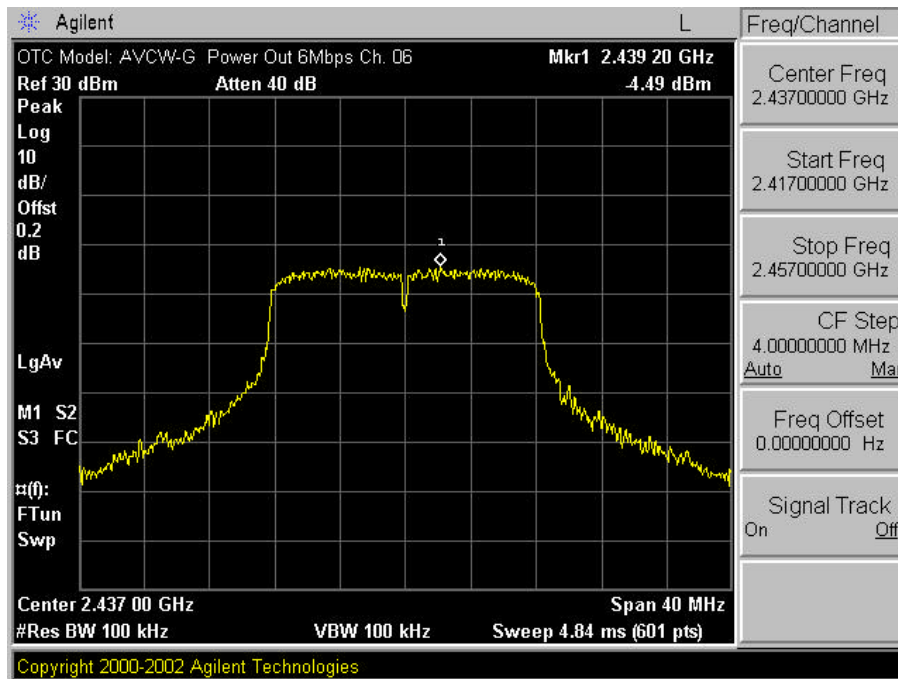
Plot A-5. Max. Output Power 6Mbps Plot – Ch. 06
