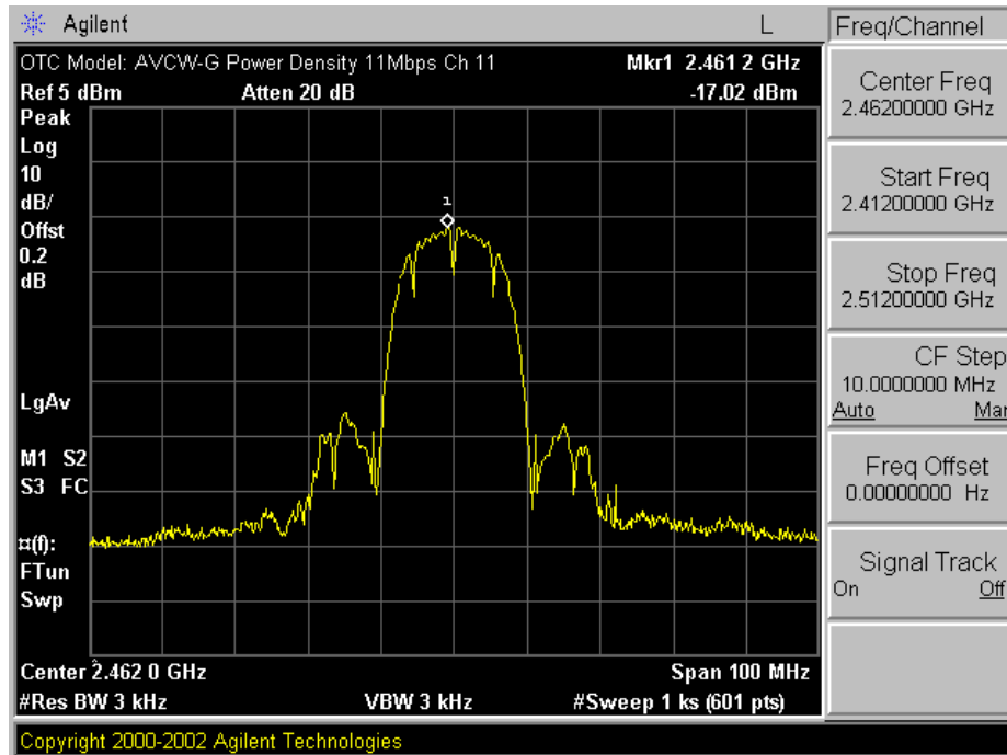
Plot A-9. Max. Power Density 11Mbps Plot – Ch. 11
