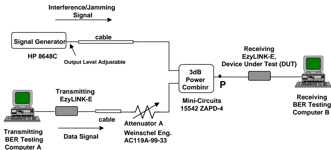
Figure 1. Processing Gain Measurement Setup for EzyLINK-E.
