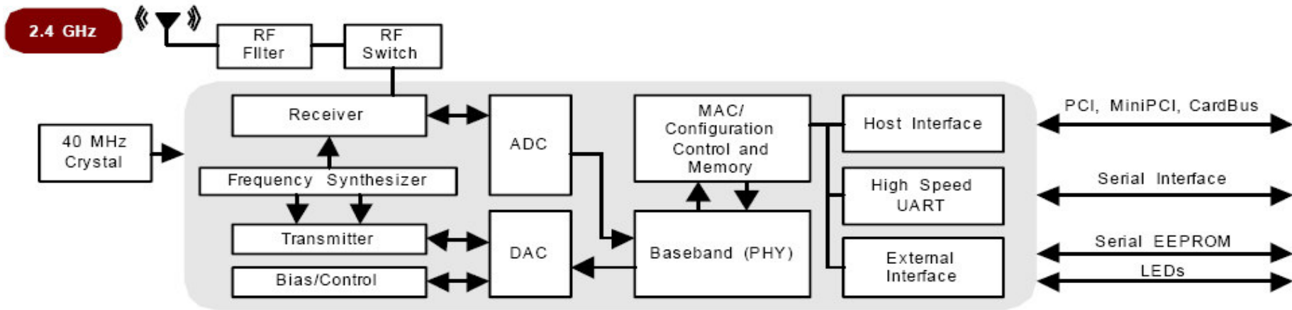
AR2413 (Block Diagram)
