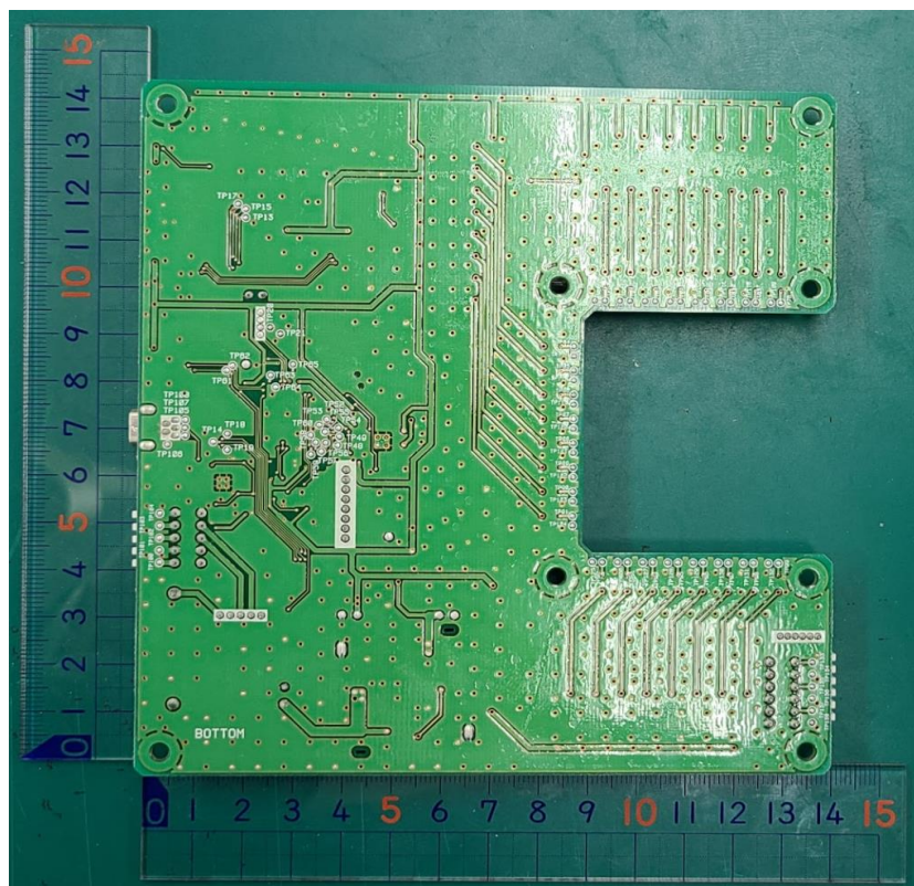
Bottom View
