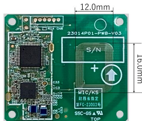
Small Antenna
