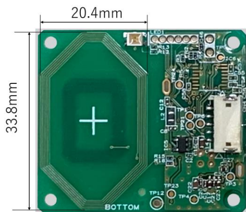
Large Antenna
