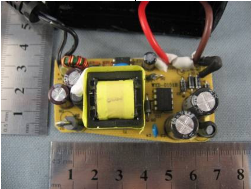
AC Adapter
