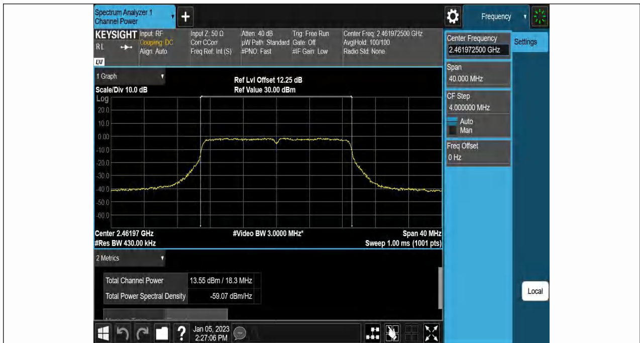
11N20SISO-Ant1-2462-----13.27-93.85-0.28
