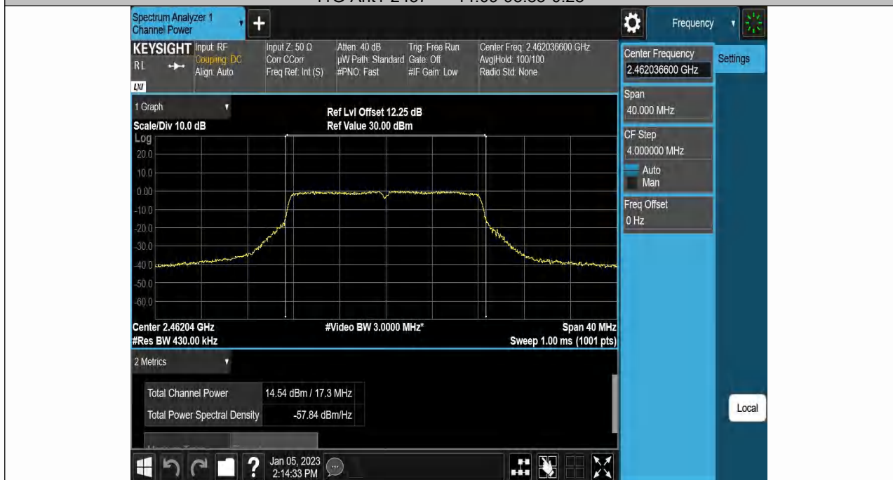
11G-Ant1-2462-----14.26-93.85-0.28
