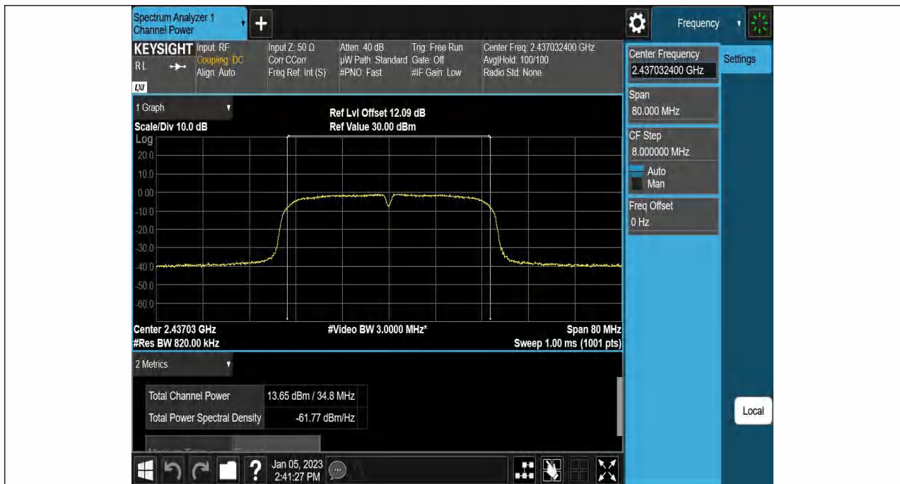
11N40SISO-Ant1-2437-----13.62-99.20-0.03
