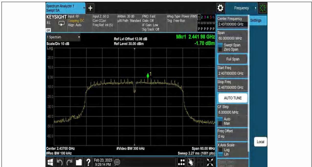
11N40SISO-Ant1-2437-0~Reference--1.70
