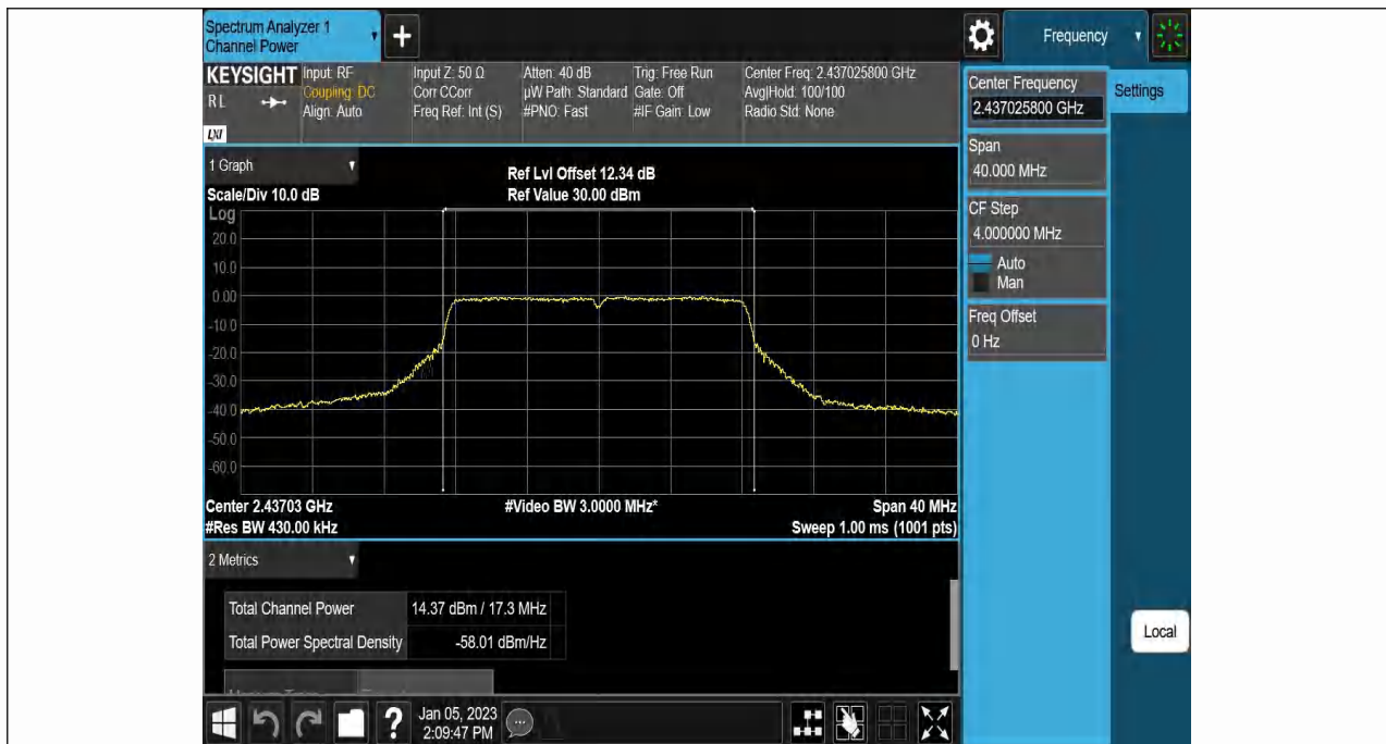
11G-Ant1-2437-----14.09-93.85-0.28
