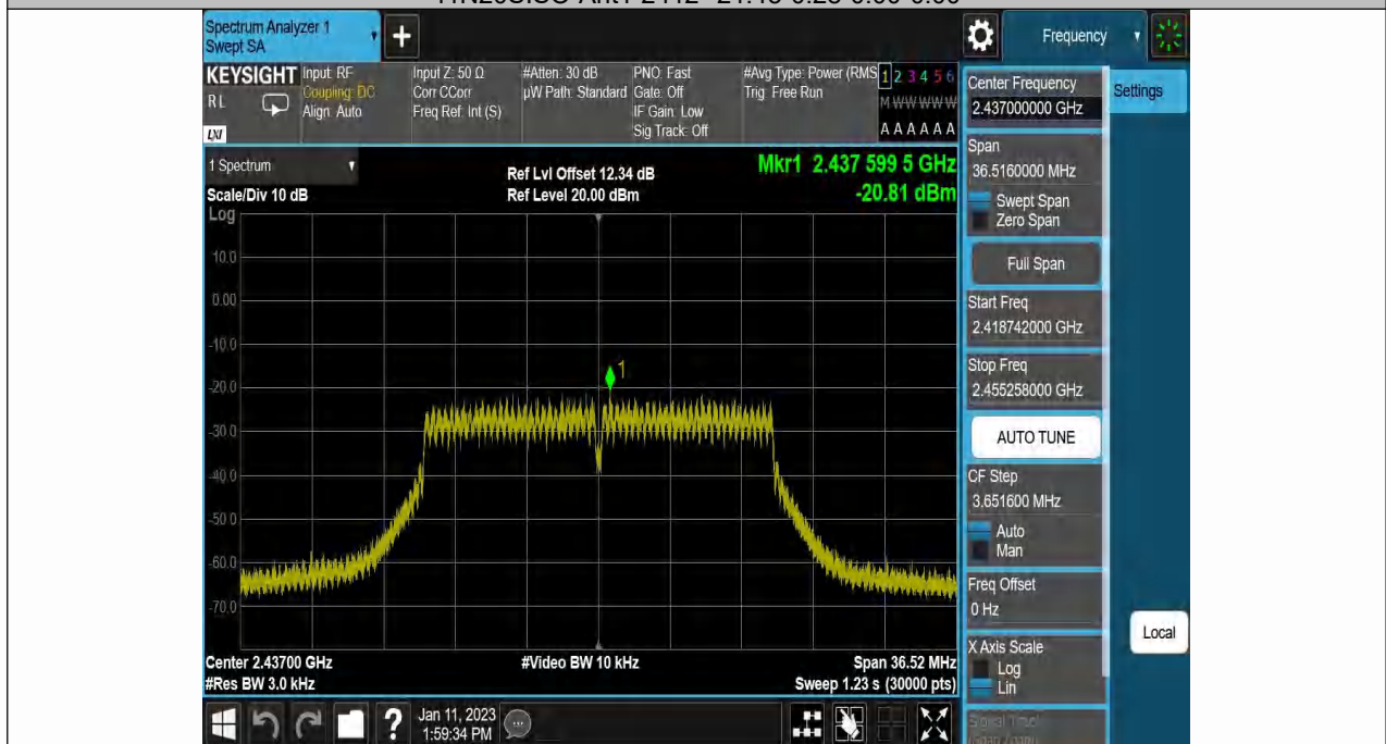
11N20SISO-Ant1-2437--21.09-0.28-0.00-0.00
