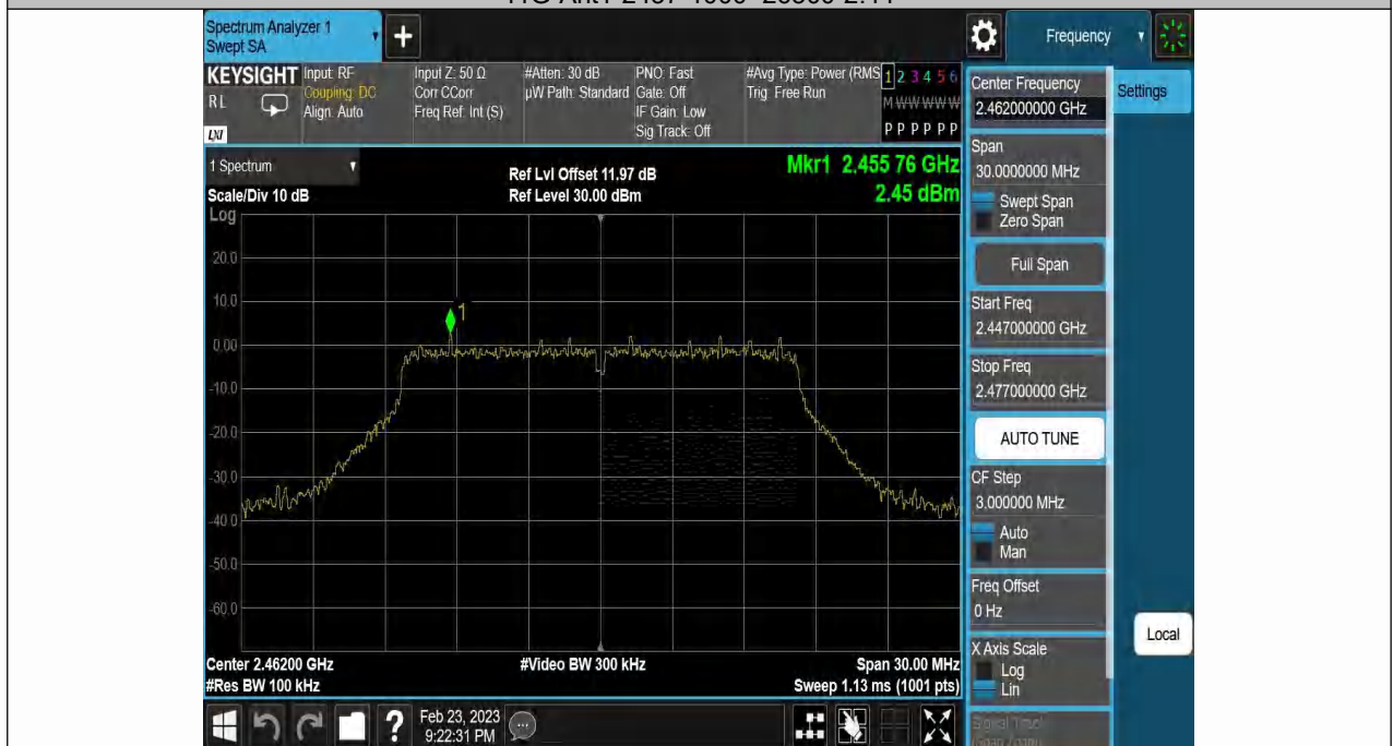
11G-Ant1-2462-0~Reference-2.45
