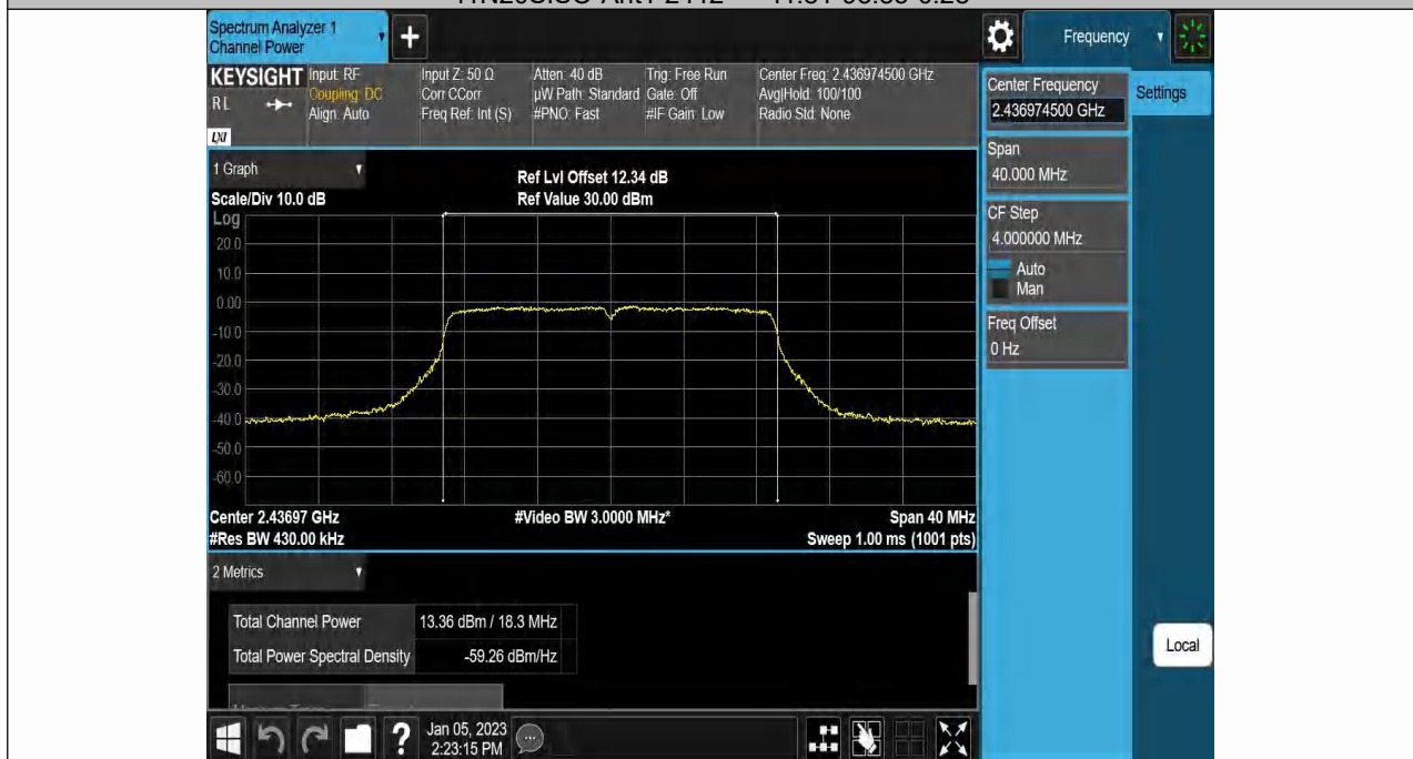
11N20SISO-Ant1-2437-----13.08-93.85-0.28
