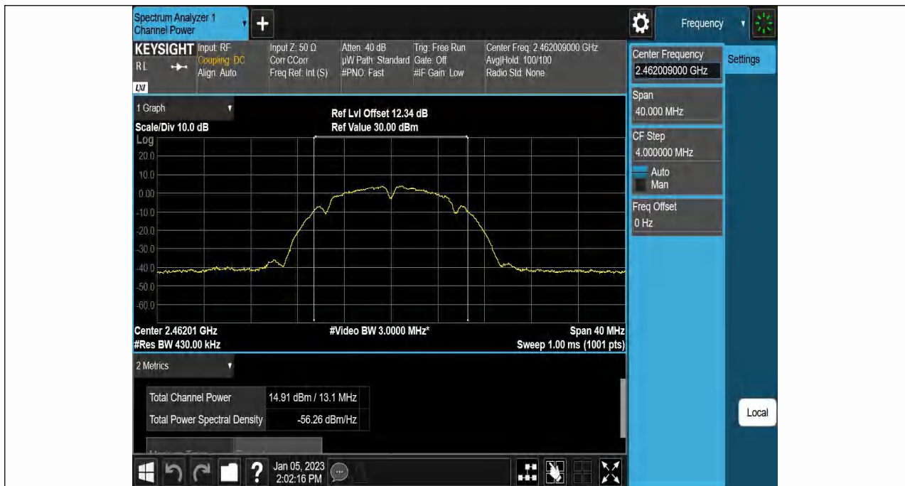
11B-Ant1-2462-----14.54-91.74-0.37
