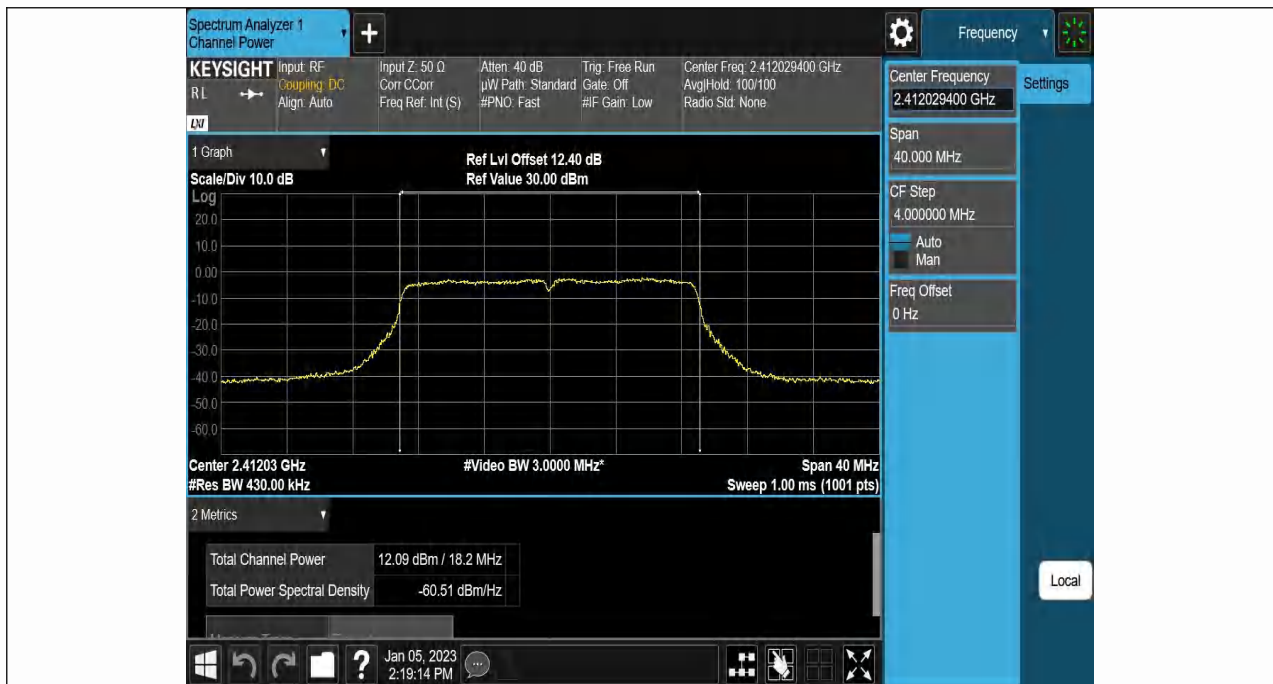
11N20SISO-Ant1-2412-----11.81-93.85-0.28
