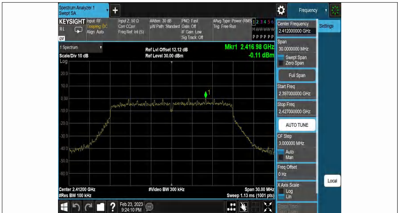
11N20SISO-Ant1-2412-0~Reference--0.11
