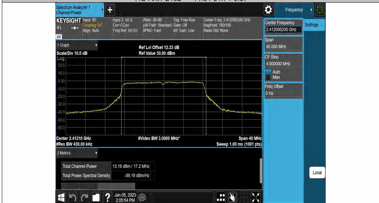
11G-Ant1-2412-----12.98-95.38-0.21
